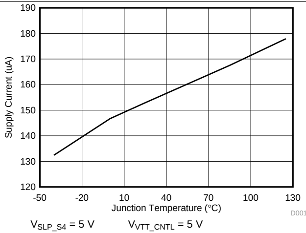
图 1. VCC_5V Supply Current vs Junction Temperature
