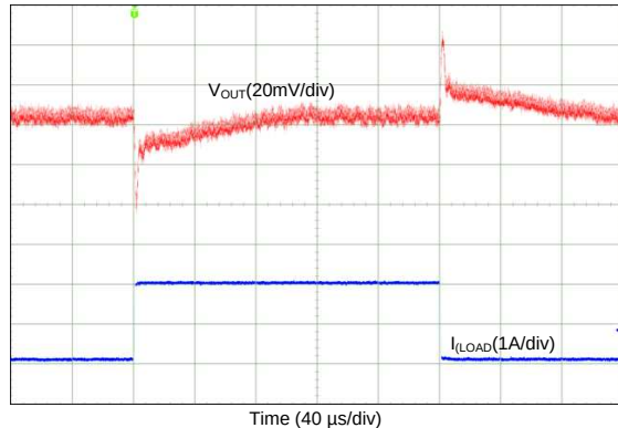
图 106. Transient Load Step Response, Forced-PWM Mode (1-Phase Output)
