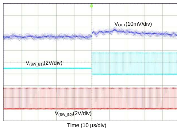
图 95. Transient from 1-Phase to 2-Phase Operation (2-Phase Output)
