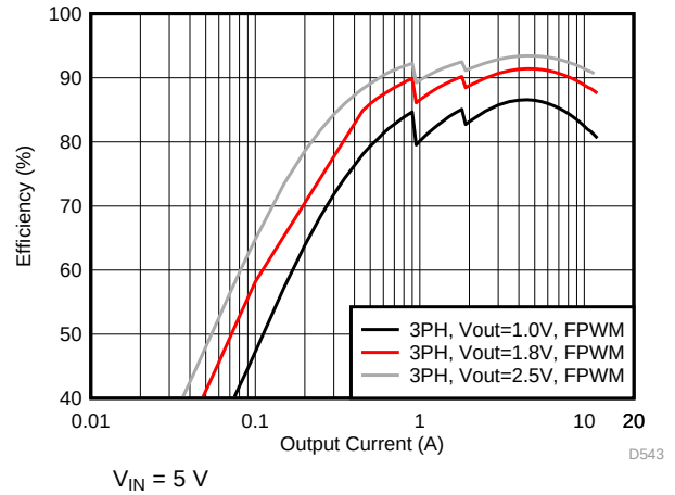
图 43. Efficiency in Forced-PWM Mode (3-Phase Output)
