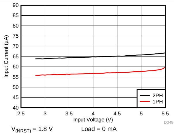
图 6. PFM Mode Current Consumption vs Input Voltage, One Regulator Enabled (2+1+1-Phase Output)
