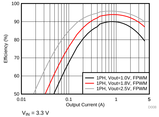
图 41. Efficiency in Forced-PWM Mode (1-Phase Output)
