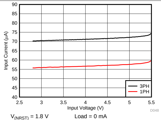
图 5. PFM Mode Current Consumption vs Input Voltage, One Regulator Enabled (3+1-Phase Output)
