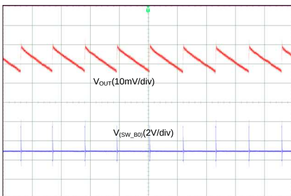
图 78. Output Voltage Ripple, PFM Mode (3-Phase Output)
