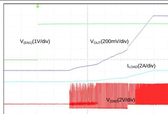
图 71. Start-Up With EN1, Forced PWM (2-Phase Output)
