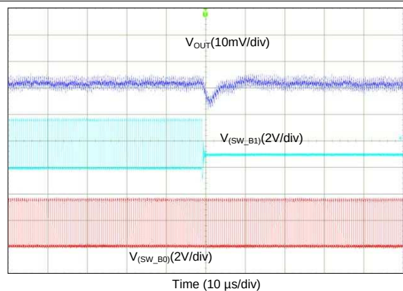
图 98. Transient from 2-Phase to 1-Phase Operation (2-Phase Output)
