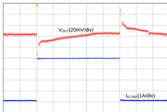
图 103. Transient Load Step Response, Forced-PWM Mode (4-Phase Output)
