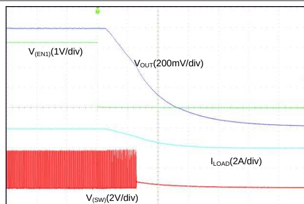
图 73. Shutdown With EN1, Forced PWM (4-Phase Output)
