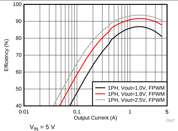
图 45. Efficiency in Forced-PWM Mode (1-Phase Output)
