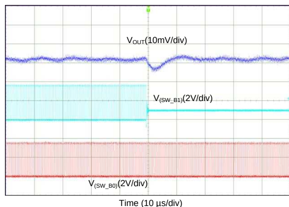
图 96. Transient from 2-Phase to 1-Phase Operation (4-Phase Output)
