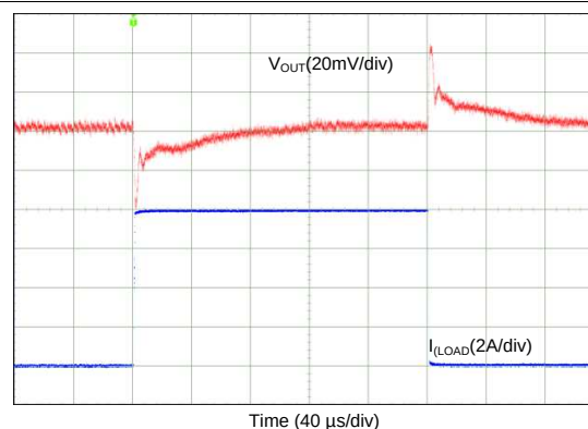
图 97. Transient from 2-Phase to 1-Phase Operation (3-Phase Output)
