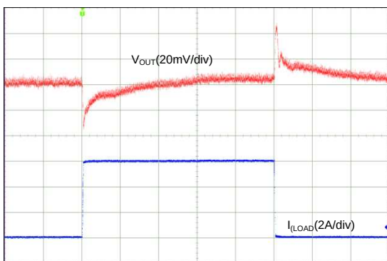
图 102. Transient Load Step Response, AUTO Mode (1-Phase Output)
