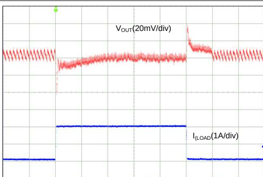
图 100. Transient Load Step Response, AUTO Mode (3-Phase Output)
