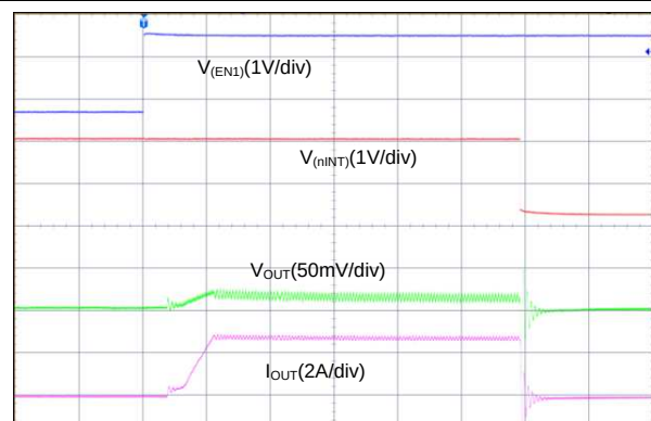
图 109. Start-Up With Short on Output (4-Phase Output)
