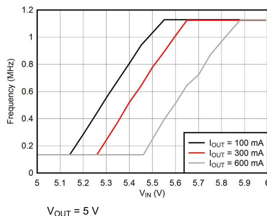
图 8-5. Frequency Foldback at T_{OFF\_MIN}
