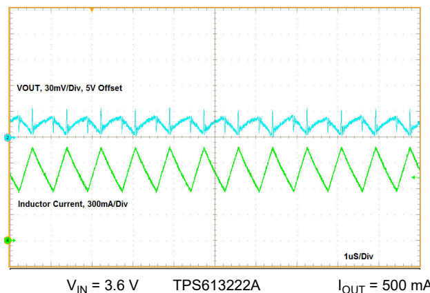
图 8-12. Switching Waveform at Heavy Load
