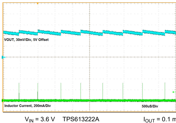
图 8-10. Switching Waveform at Light Load
