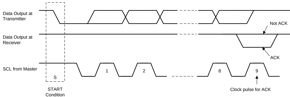
图 5-11. Acknowledge on the I 2 C Bus
