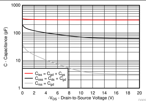
Figure 4-5. Capacitance
