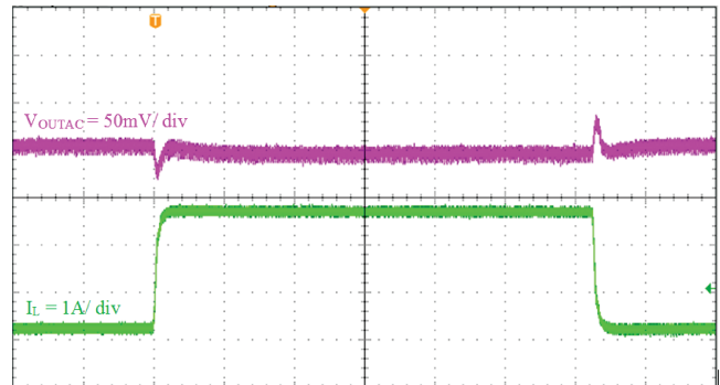
TPS565208 负载调整率
