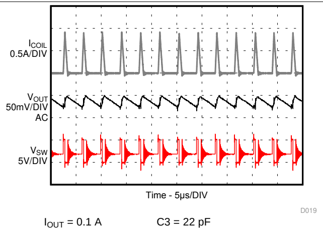
图 14. PSM Operation with A Feedforward Capacitor
