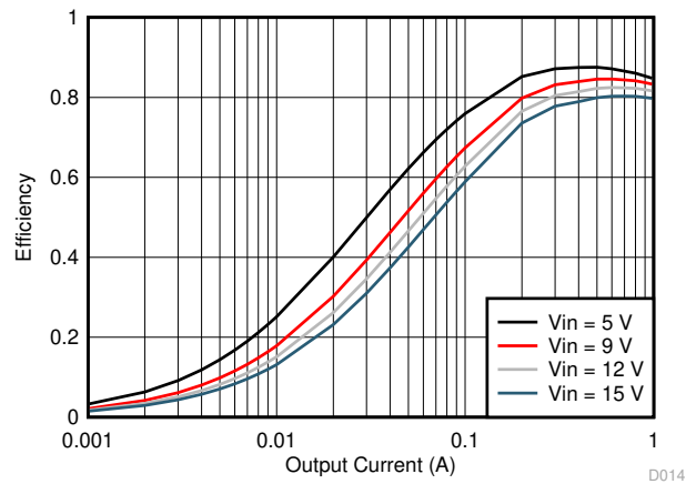
图 6-13. TPS561208 V_{OUT} = 1.05\text{ V} , Efficiency, L = 2.2\text{ }\mu\text{H}
