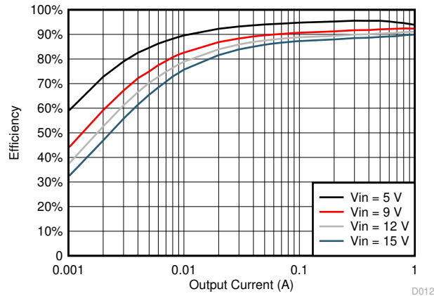
图 6-11. TPS561201 V_{OUT} = 3.3\text{ V} , Efficiency, L = 3.3\text{ }\mu\text{H}
