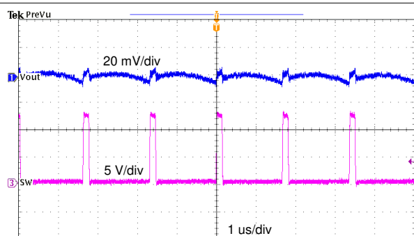
图 8-10. TPS561208 Output Voltage Ripple, I_{OUT} = 0\text{ A}
