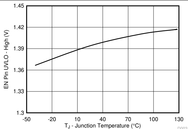
图 6-4. EN Pin UVLO High Voltage vs Junction Temperature
