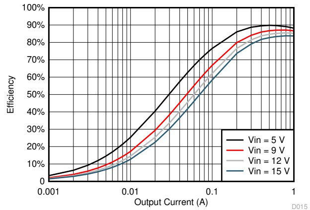
图 6-14. TPS561208 V_{OUT} = 1.5\text{ V} , Efficiency, L = 2.2\text{ }\mu\text{H}
