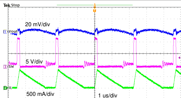
图 8-8. TPS561201 Output Voltage Ripple, I_{OUT} = 0.25\text{ A}
