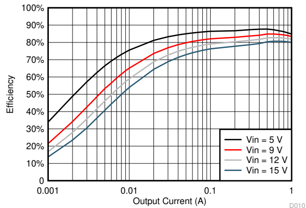
图 6-9. TPS561201 V_{OUT} = 1.05 V, Efficiency, L = 2.2 \mu H
