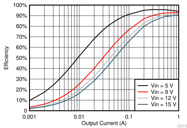
图 6-15. TPS561208 V_{OUT} = 3.3\text{ V} , Efficiency, L = 3.3\text{ }\mu\text{H}
