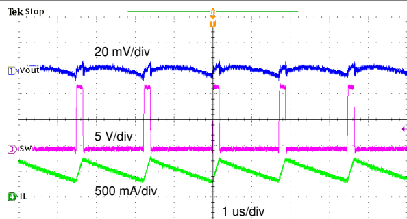
图 8-9. TPS561201 Output Voltage Ripple, I_{OUT} = 1\text{ A}
