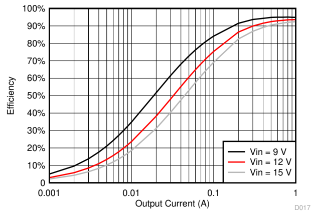
图 6-16. TPS561208 V_{OUT} = 5\text{ V} , Efficiency, L = 4.7\text{ }\mu\text{H}
