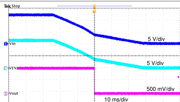
图 8-16. TPS561201 Shutdown Relative to V_I
