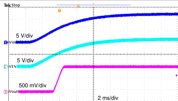
图 8-14. TPS561201 Start-Up Relative to V_I
