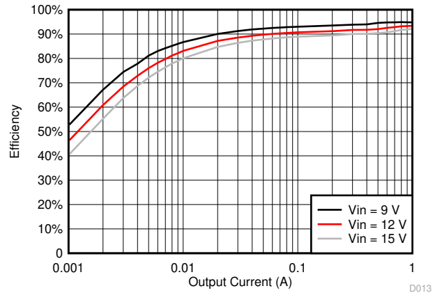
图 6-12. TPS561201 V_{OUT} = 5\text{ V} , Efficiency, L = 4.7\text{ }\mu\text{H}
