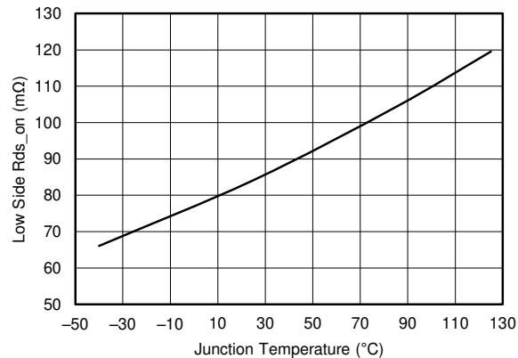
图 6-6. Low-Side R_{ds-on} vs Junction Temperature
