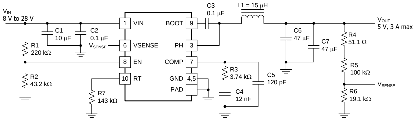
Figure 21. Typical Application Schematic, TPS54335-2A
