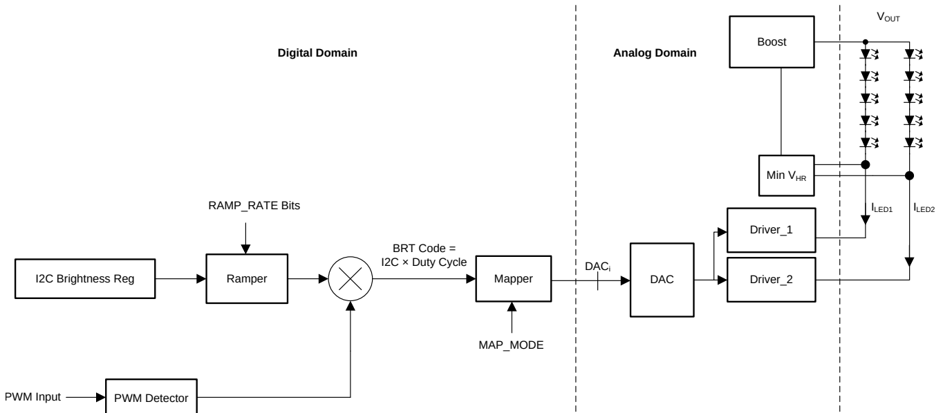
图 35. (I 2 C + PWM) Brightness Control, PWM Ramper Disabled
