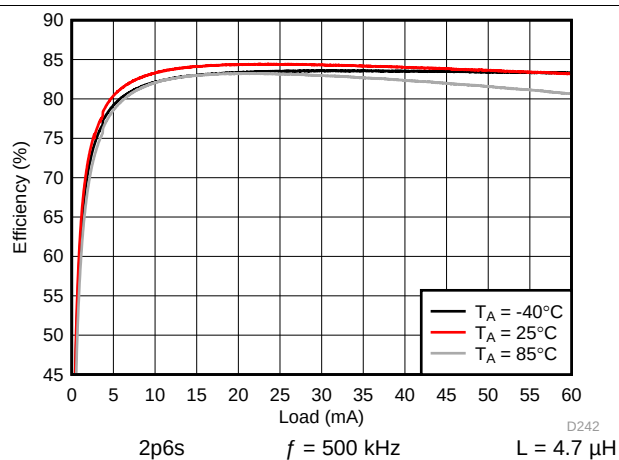
图 110. Backlight System Efficiency
