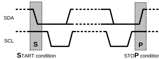
图 44. Start and Stop Conditions
