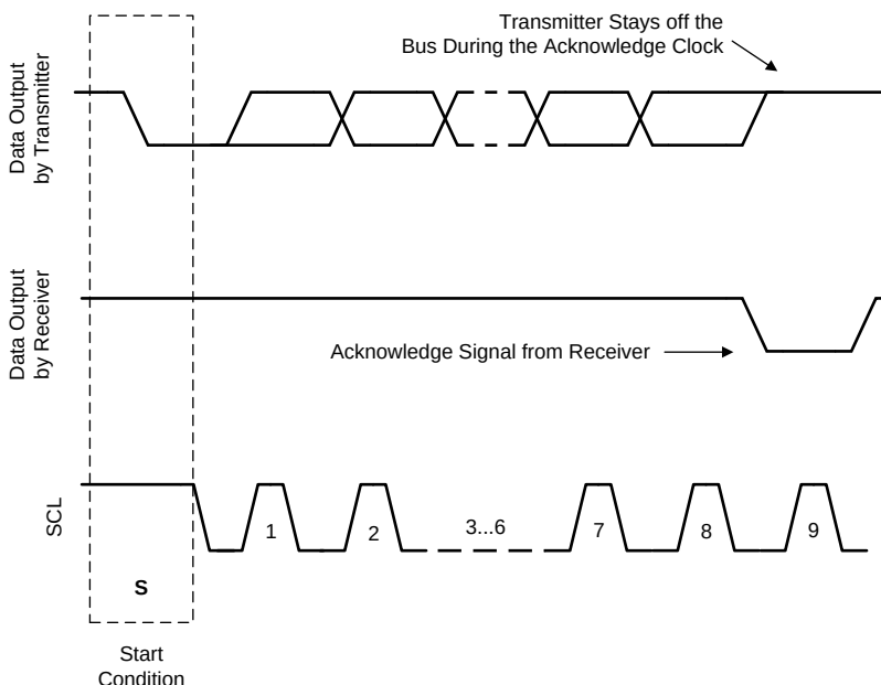
图 43. Acknowledge Signal
