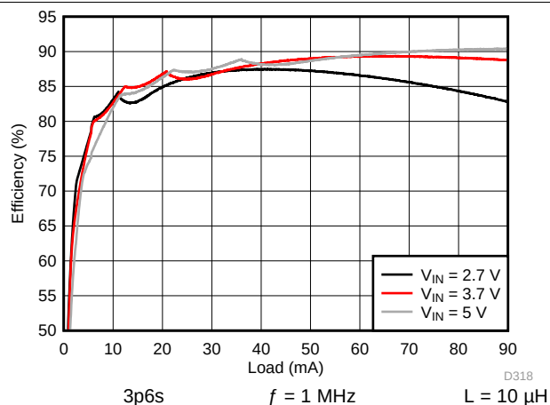
图 130. Backlight System Efficiency
