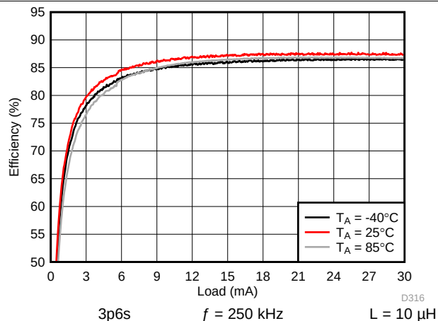
图 128. Backlight System Efficiency
