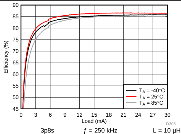
图 118. Backlight System Efficiency
