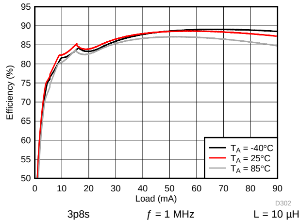
图 116. Backlight System Efficiency
