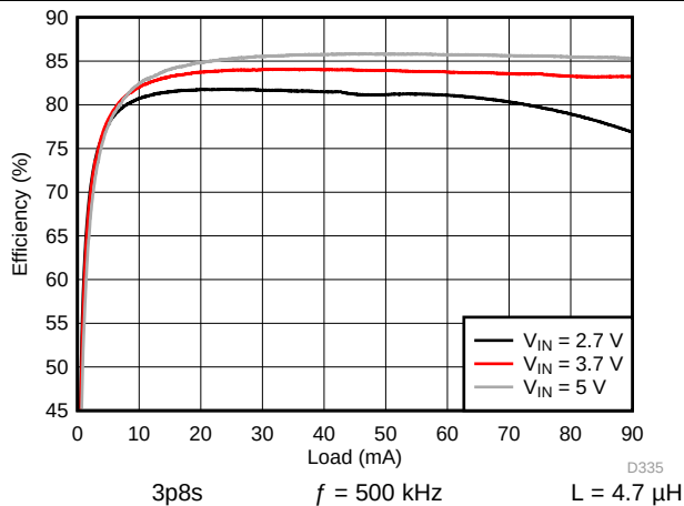
图 147. Backlight Boost Efficiency
