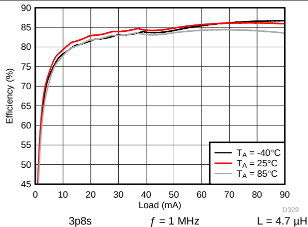
图 141. Backlight Boost Efficiency
