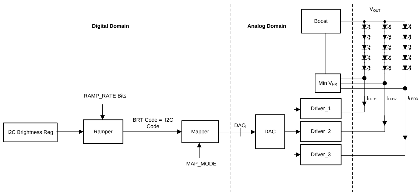
图 34. I 2 C Only Brightness Control
