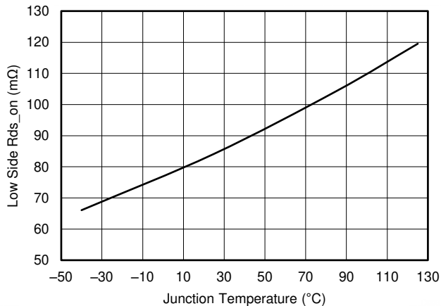
图 5-6. Low-Side R_{ds-on} vs Junction Temperature
