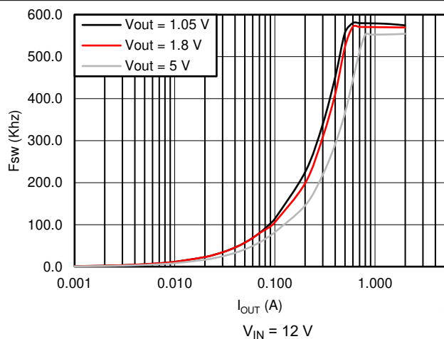
图 5-8. TPS562201 Switching Frequency vs Output Current
