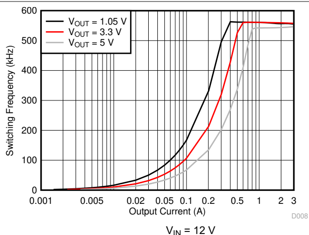
图 5-8. TPS563201 Switching Frequency vs Output Current
