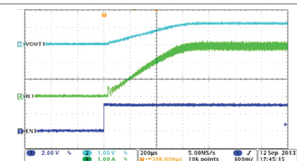
图 8-4. PSM Mode Buck1, Soft-Start With Full Load
