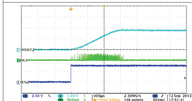
图 8-5. PSM Mode Buck2, Soft-Start with No Load
