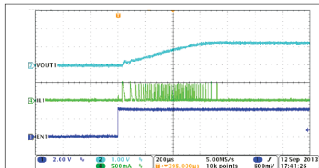
图 8-3. PSM Mode Buck1, Soft-Start with No Load
