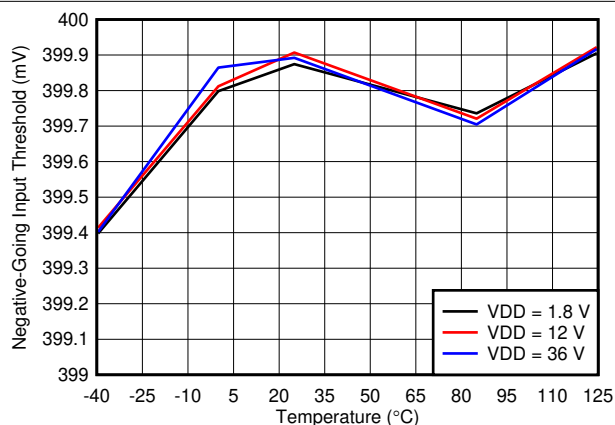
图 5-5. SENSE Negative Input Threshold Voltage ( V_{IT-} ) vs Temperature
