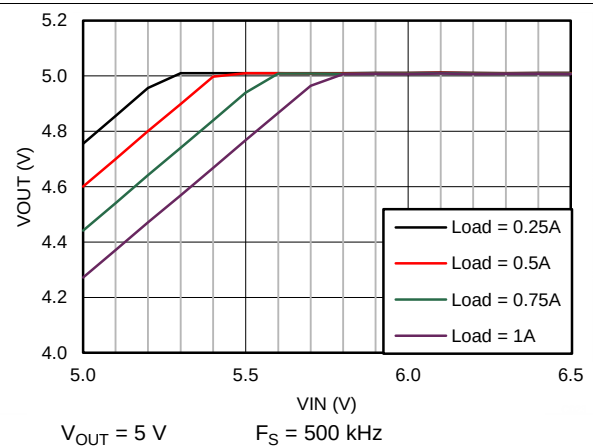
Figure 56. Dropout Curve
