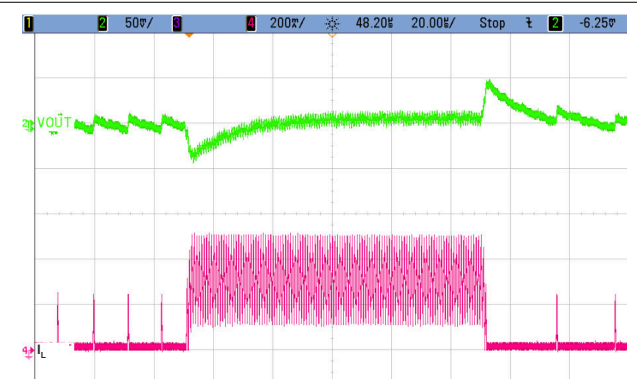
图 9-19. Load Transient Response; 5 mA to 290 mA
