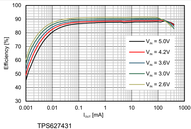
图 9-4. Efficiency vs Load Current; V_{OUT} = 1.9\text{ V}
