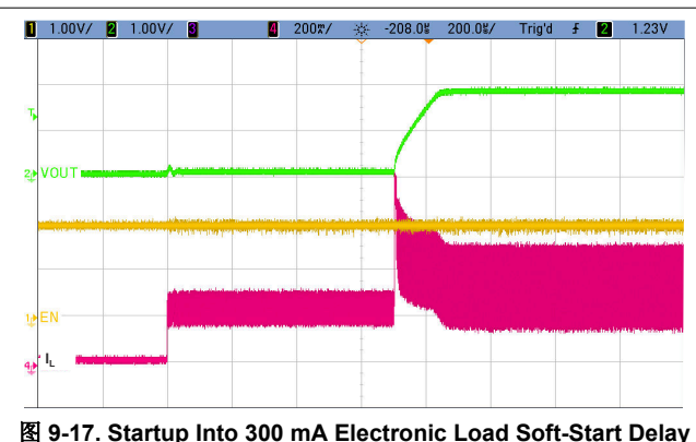
图 9-17. Startup Into 300 mA Electronic Load Soft-Start Delay
