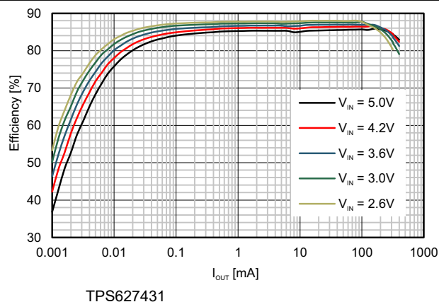
图 9-6. Efficiency vs Load Current; V_{OUT} = 1.4\text{ V}
