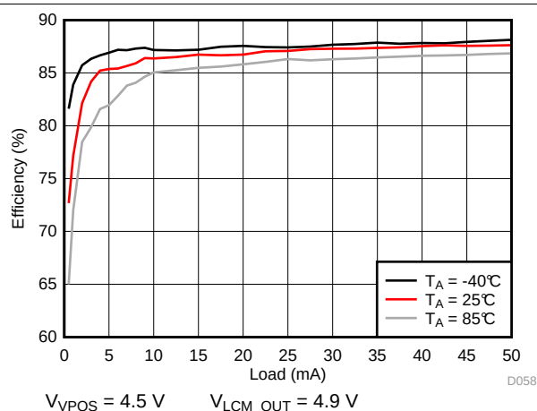
Figure 76. VPOS Efficiency
