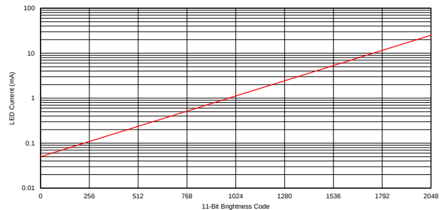
Figure 20. Response of LED Current vs Brightness Code on a Log Y Axis
