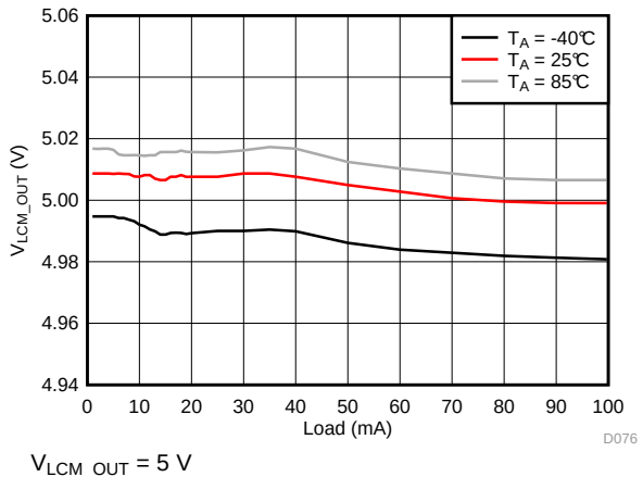
Figure 94. V_{LCM\_OUT} Load Regulation
