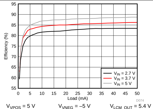
Figure 92. VPOS/VNEG Efficiency
