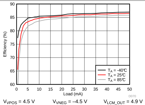
Figure 88. VPOS/VNEG Efficiency
