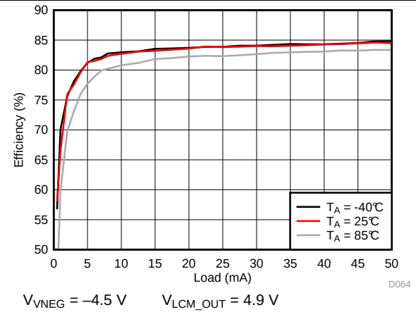
Figure 82. VNEG Efficiency
