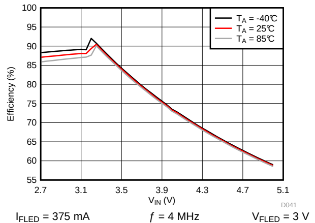
Figure 112. Torch System Efficiency
