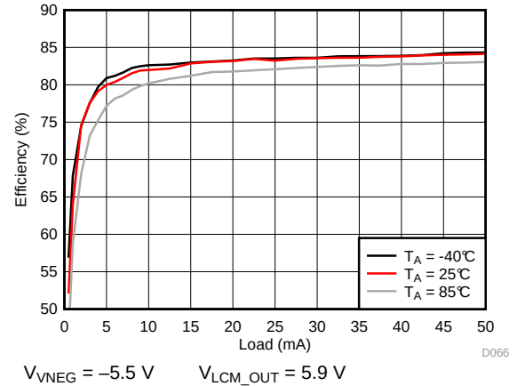
Figure 84. VNEG Efficiency
