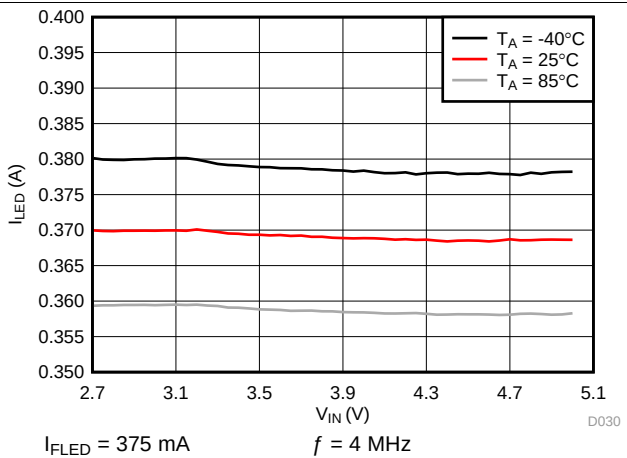
Figure 15. Flash LED Current
