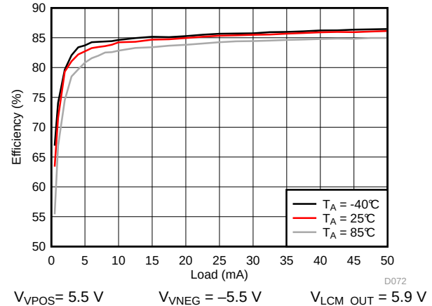
Figure 90. VPOS/VNEG Efficiency
