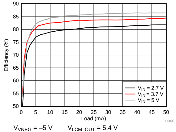
Figure 86. VNEG Efficiency
