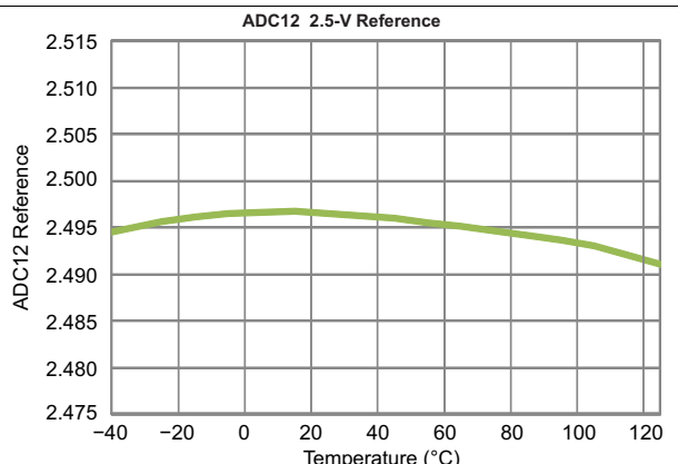
Figure 5-14. ADC12 2.5-V Reference vs Temperature
