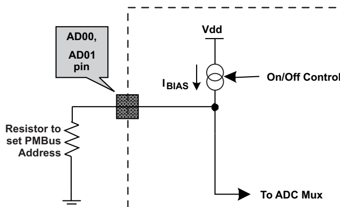
Figure 6-18. PMBus Address Detection Method
