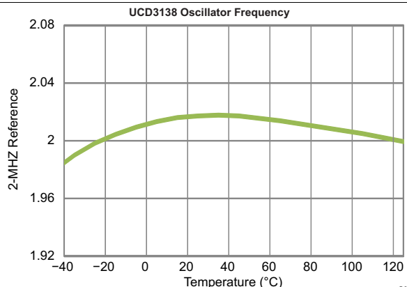
Figure 5-16. UCD3138A Oscillator Frequency (2-MHz Reference, Divided Down from 250 MHz) vs Temperature
