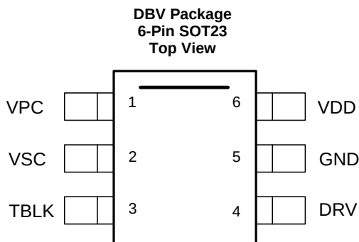
Pin Functions
