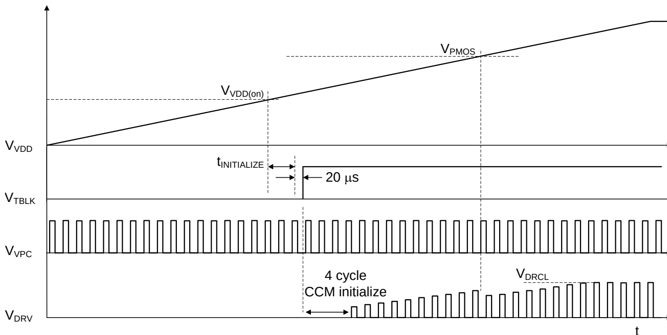
Figure 13. Start-Up Operation
