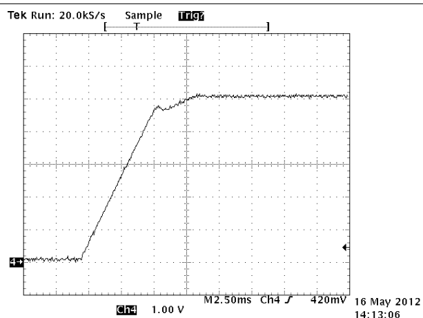
图 8-5. Output at Startup at 230-V RMS (5-Ω Load)
