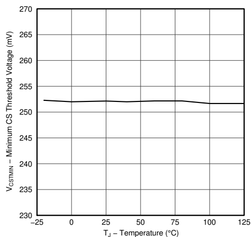
图 6-5. Minimum CS Threshold Voltage vs. Temperature
