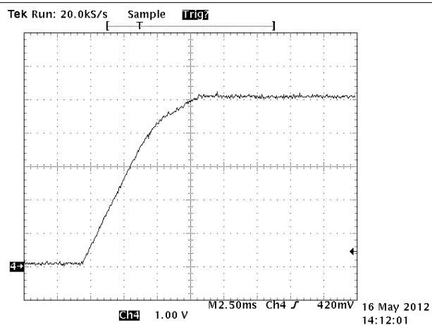
图 8-3. Output at Startup at 115-V RMS (5-Ω Load)
