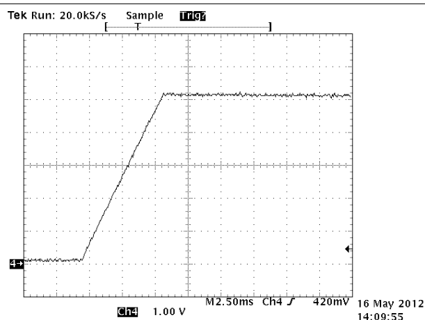
图 8-4. Output at Startup at 230-V RMS (No Load)
