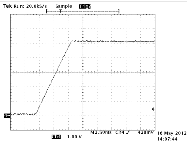
图 8-2. Output at Startup at 115-V RMS (No Load)
