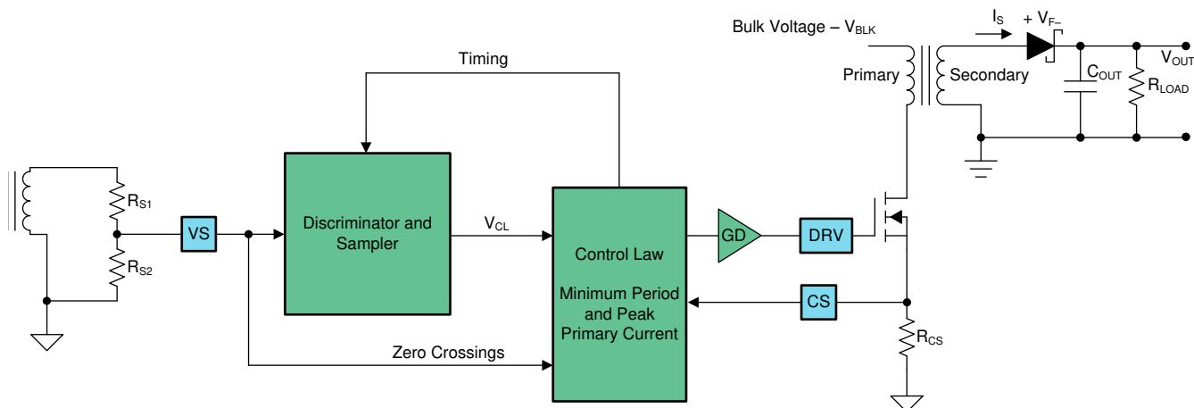
图 7-1. Simplified Flyback Convertor (with the main voltage regulation blocks)
