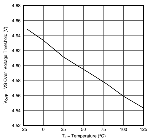
图 6-9. Overvoltage Threshold vs. Temperature
