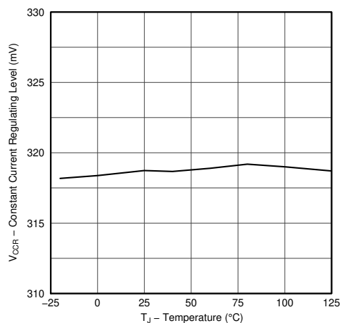
图 6-6. Constant-Current Regulating Level vs. Temperature
