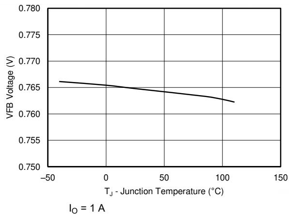
图 6-3. Vfb Voltage vs Junction Temperature
