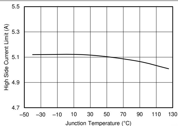
图 7-21. Buck1 High-Side Current Limit vs Temperature
