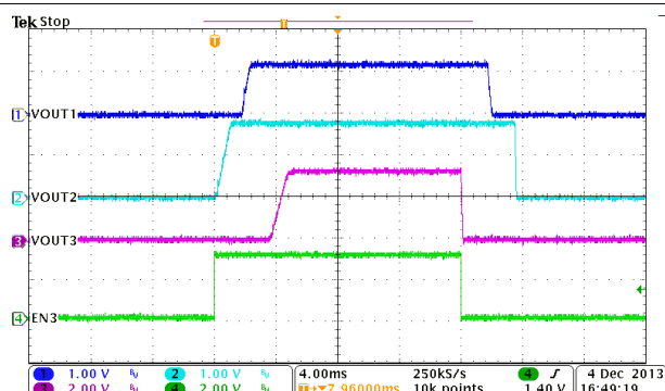
图 9-30. Automatic Power Sequencing, MODE = EN2 = HIGH, EN1 = LOW
