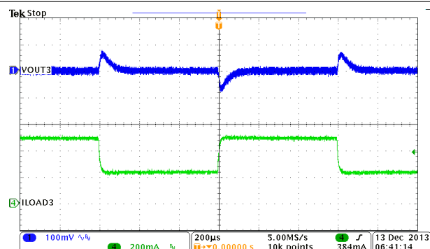
图 9-18. Buck3, Load Transient, 0.25 to 0.5 A SR = 0.25 A/µs
