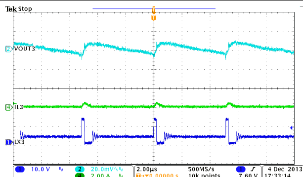
图 9-12. Buck3, Steady State Operation at Light Load
