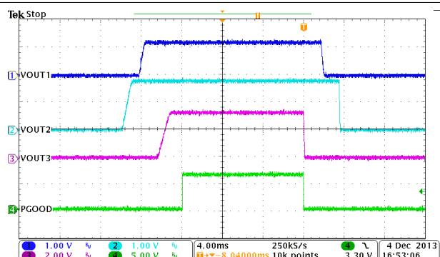
图 9-31. Automatic Power Sequencing, MODE = EN2 = HIGH, EN1 = LOW
