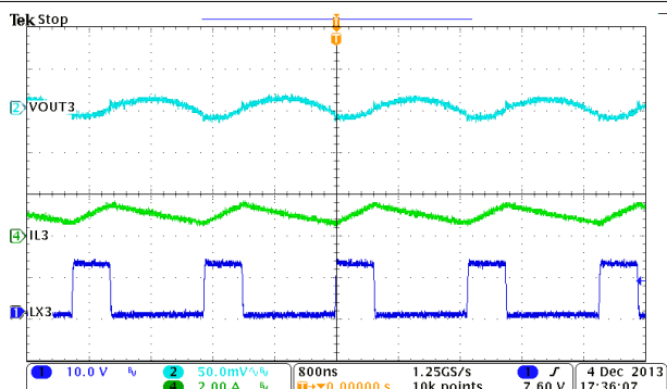
图 9-13. Buck3, Steady State Operation at Full Load
