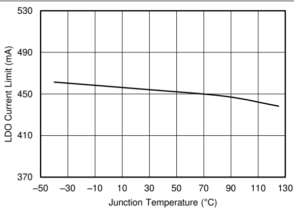
图 7-23. LDO Current Limit vs Temperature
