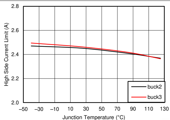
图 7-22. Buck2, 3 High-Side Current Limit vs Temperature
