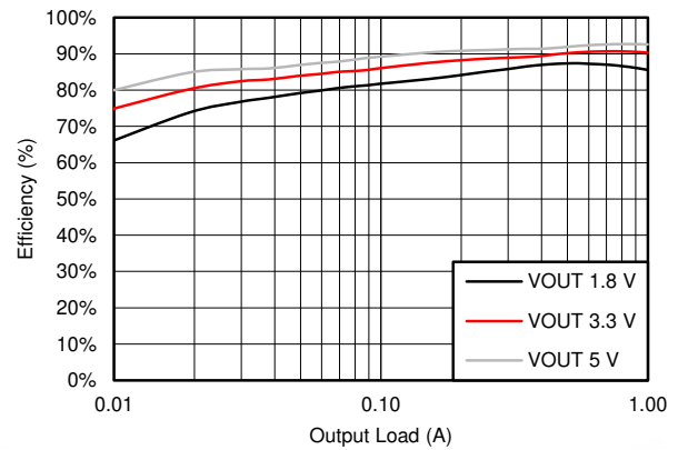
图 7-2. BUCK2 Efficiency
