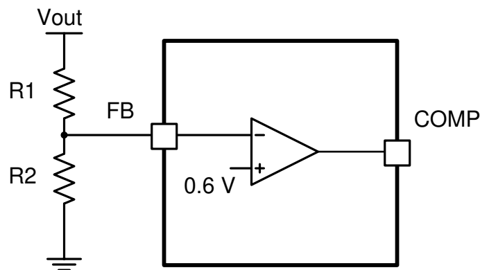
图 8-1. Voltage Divider Circuit
