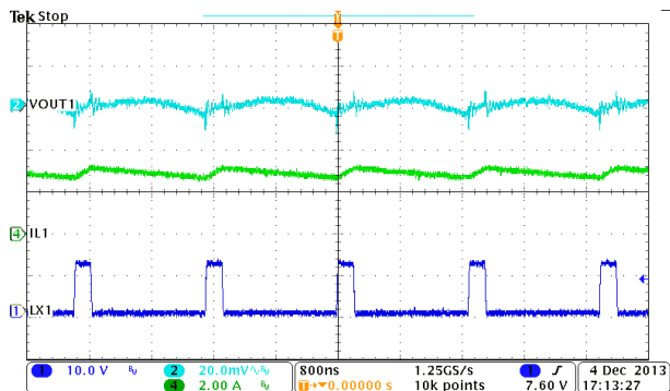
图 9-9. Buck1, Steady State Operation at Full Load
