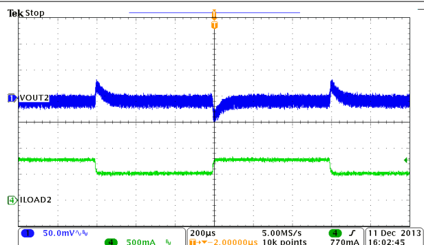
图 9-17. Buck2, Load Transient, 0.5 to 0.75 A SR = 0.25 A/µs
