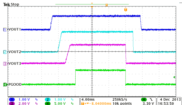
图 9-27. Automatic Power Sequencing, MODE = EN1 = EN2 = HIGH
