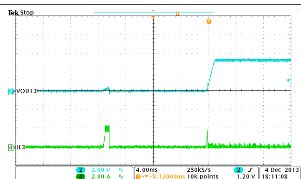
图 9-25. Buck3, Hiccup and Recovery
