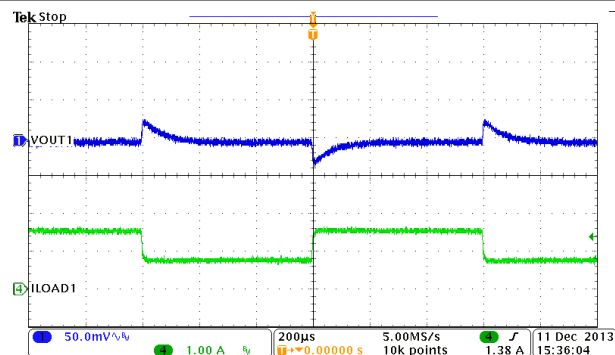
图 9-14. Buck1, Load Transient, 0.75 to 1.5 A SR = 0.25 A/µs
