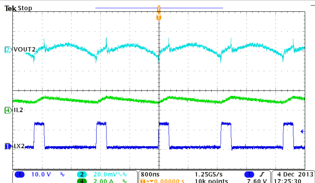
图 9-11. Buck2, Steady State Operation at Full Load
