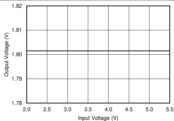
图 7-12. LDO2, Line Regulation
