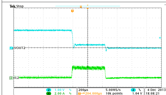
图 9-22. Buck2, OCP
