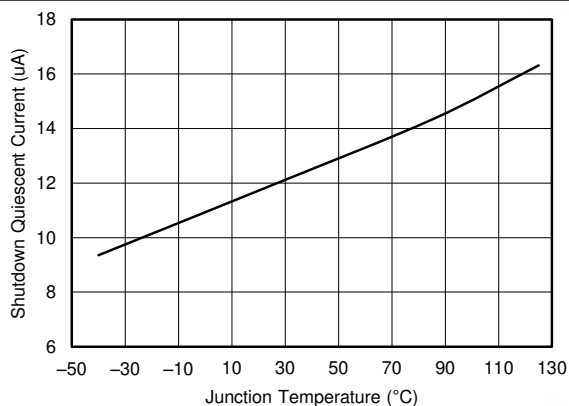
图 7-15. Shutdown Quiescent Current vs Temperature
