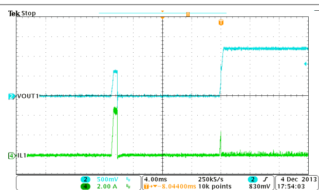
图 9-21. Buck1, Hiccup and Recovery
