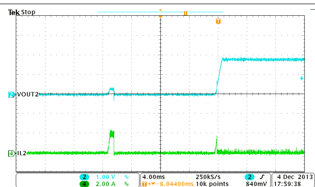
图 9-23. Buck2, Hiccup and Recovery
