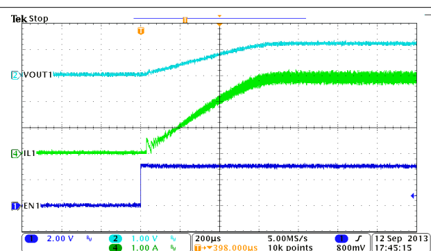
图 9-3. BUCK1, Soft-Start With Full Load
