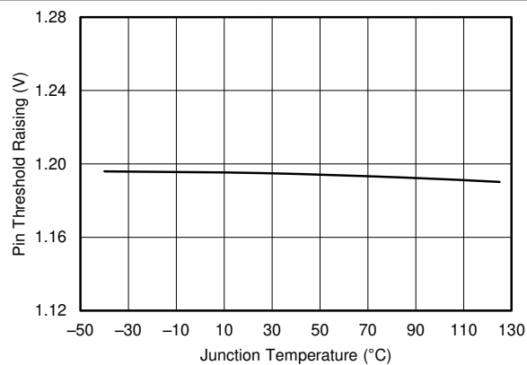
图 7-18. EN Pin Threshold Rising vs Temperature
