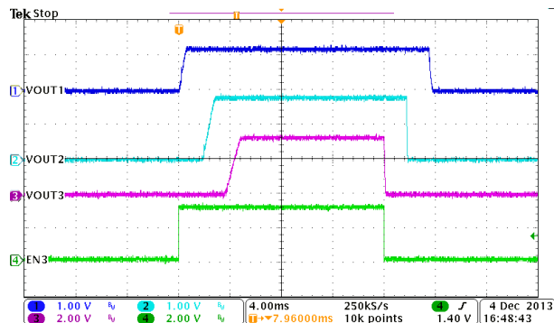
图 9-26. Automatic Power Sequencing, MODE = EN1 = EN2 = HIGH
