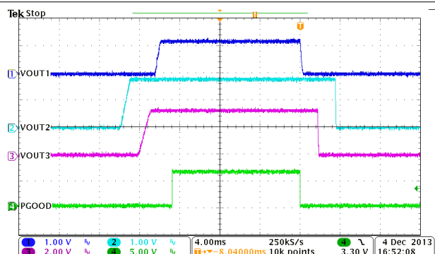
图 9-29. Automatic Power Sequencing, MODE = EN1 = HIGH, EN2 = LOW
