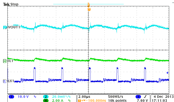
图 9-8. Buck1, Steady State Operation at Light Load
