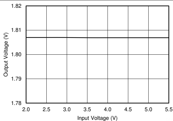
图 7-11. LDO1, Line Regulation
