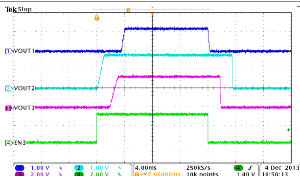
图 9-28. Automatic Power Sequencing, MODE = EN1 = HIGH, EN2 = LOW
