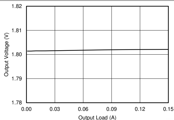
图 7-10. LDO2, Load Regulation
