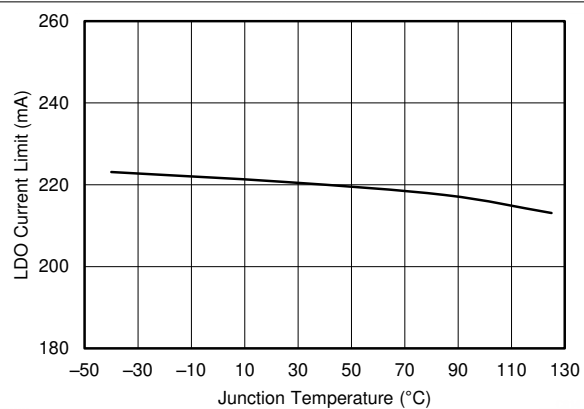
图 7-24. LDO2 Current Limit vs Temperature
