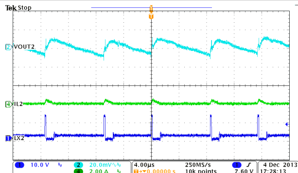
图 9-10. Buck2, Steady State Operation at Light Load
