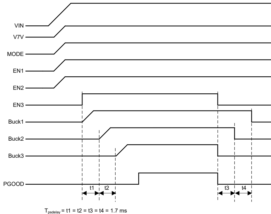
图 8-4. Automatic Power Sequencing
