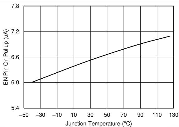
图 7-17. EN Pin Pullup Current vs Temperature, EN = 1.5 V
