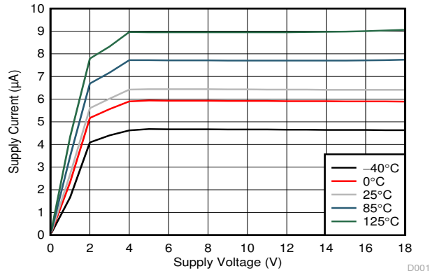
图 6-2. Supply Current ( I_{DD} ) vs Supply Voltage ( V_{DD} )
