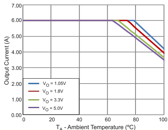
Figure 16. OUTPUT CURRENT vs AMBIENT TEMPERATURE
