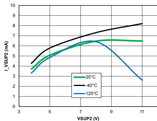
图 7-7. Open-Load Supply Current Buck2 = 3.3 V EXTSUP Pin Open
