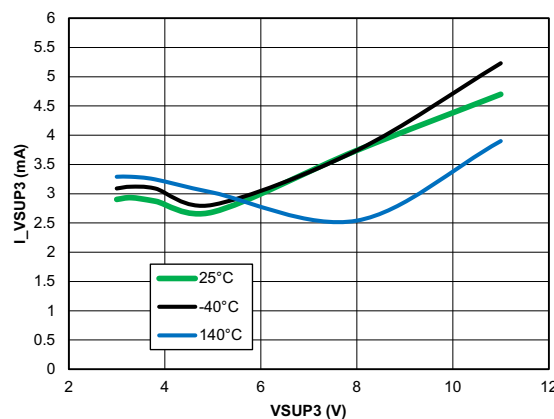
图 7-8. Open-Load Supply Current Buck3 = 1.2 V EXTSUP Pin Open
