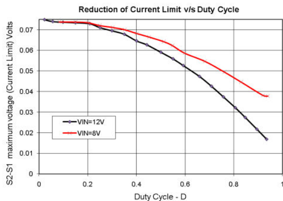
图 7-2. Reduction of Current Limit vs Duty Cycle
