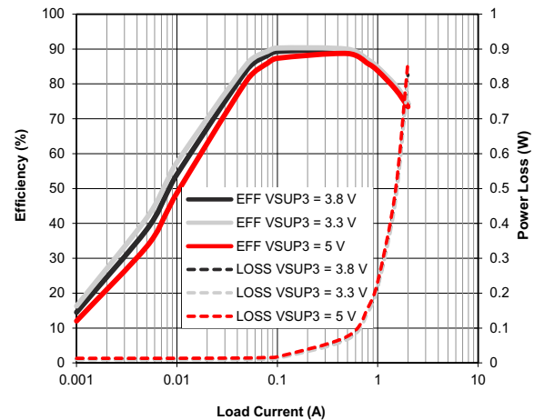
图 9-5. Efficiency Buck3 = 1.2 V At 25°C L = 3.3 \mu H , C = 30 \mu F , COMP2 Pin To Ground EXTSUP Pin Open, Measured Buck3 Output Power With Respect To VSUP3 Input Power
