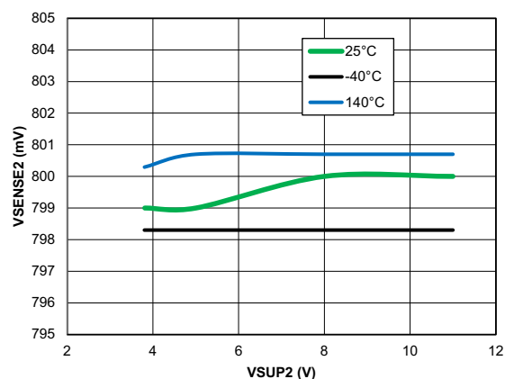
图 7-5. Open-Load Line Regulation Buck2 = 3.3 V EXTSUP Pin Open
