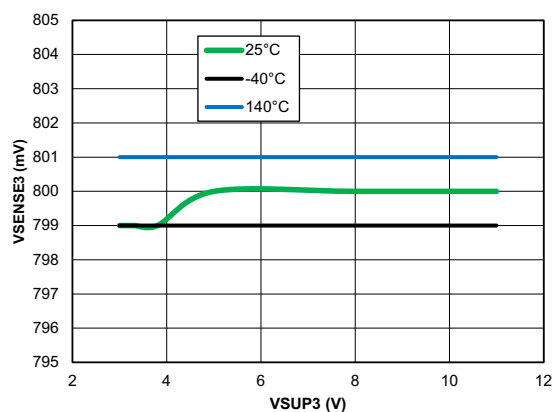
图 7-6. Open-Load Line Regulation Buck3 = 1.2 V EXTSUP Pin Open
