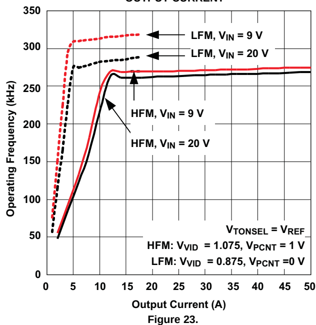
OPERATING FREQUENCY vs OUTPUT CURRENT
