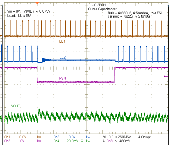
Figure 43. PCNT Toggle: V_{IN} = 9\text{ V}
