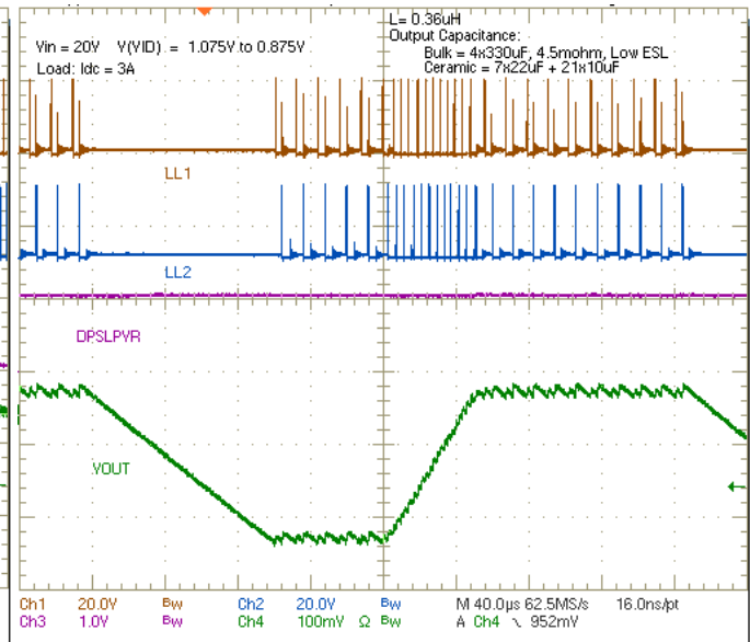
Figure 41. VID Change from 1.075 V to 0.875 V, I_{DC} = 3\text{ A}
