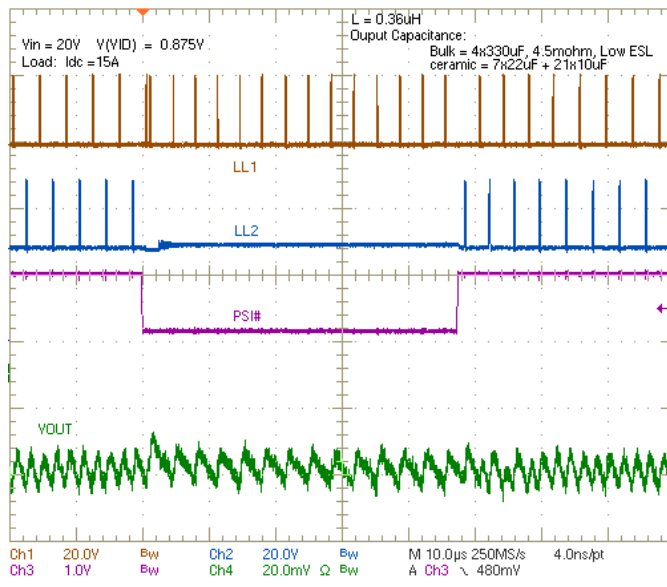
Figure 42. PCNT Toggle: V_{IN} = 20\text{ V}
