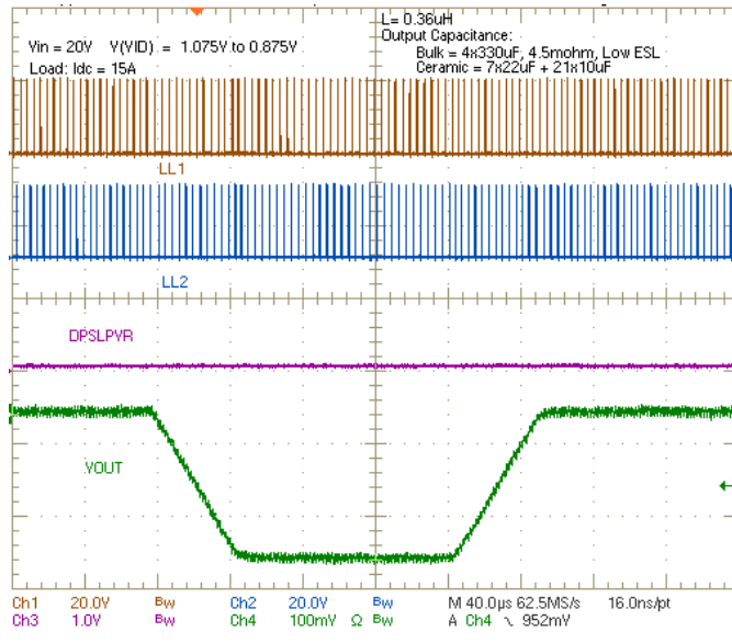
Figure 40. VID Change from 1.075 V to 0.875 V, I_{DC} = 15\text{ A}
