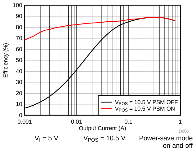
图 8. Boost Converter ( V_{POS} ) Efficiency vs Output Current
