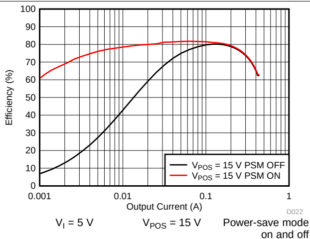
图 35. Boost Converter ( V_{POS} ) Efficiency vs Output Current
