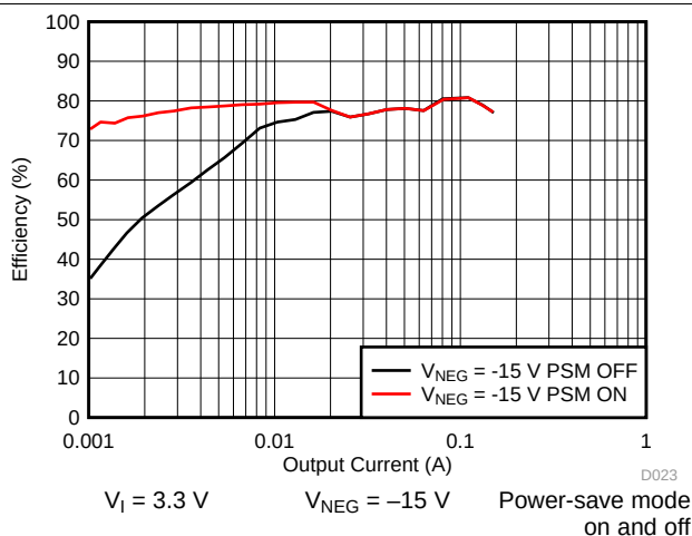
图 36. Inverting Converter ( V_{NEG} ) Efficiency vs Output Current
