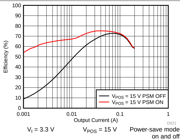
图 34. Boost Converter ( V_{POS} ) Efficiency vs Output Current
