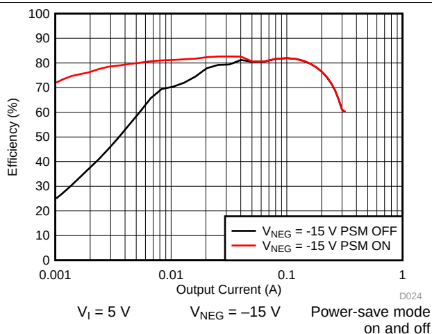
图 37. Inverting Converter ( V_{NEG} ) Efficiency vs Output Current
