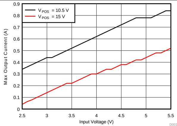
图 1. Boost Converter ( V_{\text{POS}} ) Maximum Output Current vs Input Voltage
