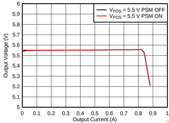
图 30. Boost Converter ( V_{POS} ) Output Voltage vs Output Current
