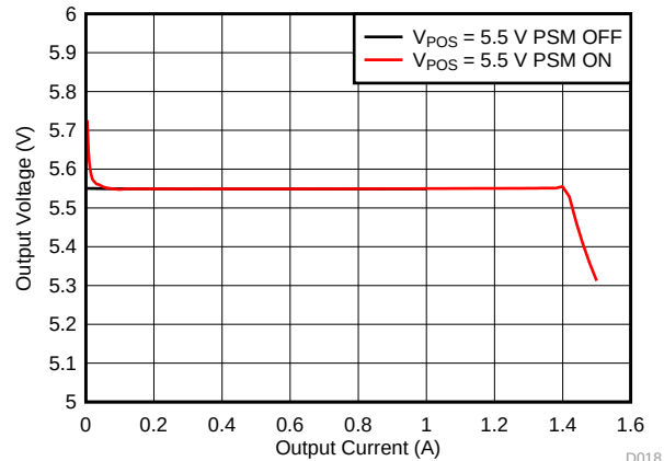
图 31. Boost Converter ( V_{POS} ) Output Voltage vs Output Current
