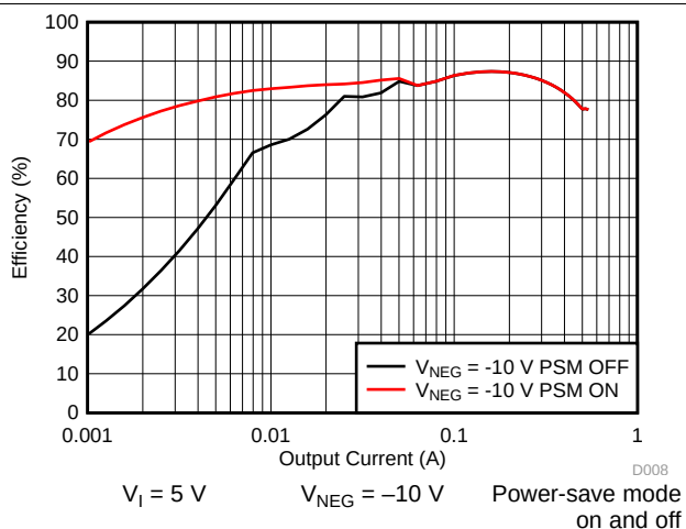
图 10. Inverting Converter ( V_{NEG} ) Efficiency vs Output Current
