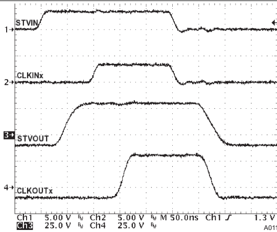
图 1. Propagation Delay, Charge Sharing Disabled
