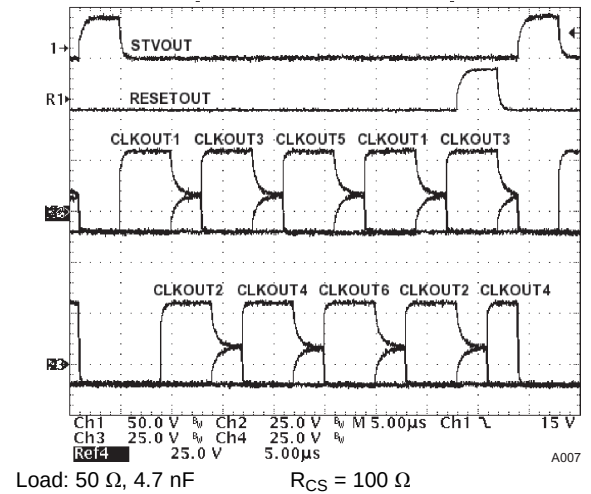
图 20. 3-Channel Charge Sharing Outputs
