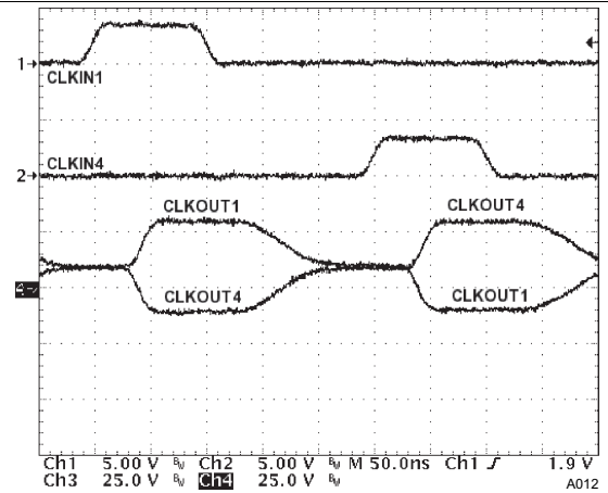
图 2. Propagation Delay, Charge Sharing Enabled
