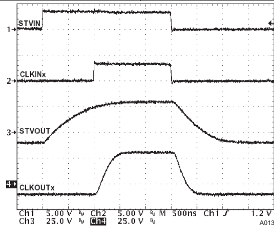
图 1. Propagation Delay, Charge Sharing Disabled
