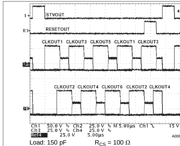
图 19. 3-Channel Charge Sharing Outputs
