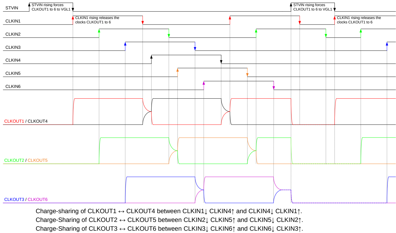
图 6. TPS65197: 2-Channel Charge-Sharing (CS_SEL = 2.8 V...6.5 V)
