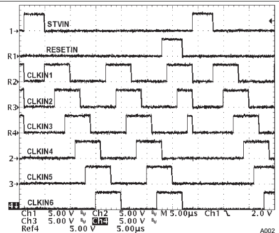
图 12. No Charge Sharing Input Signals
