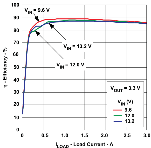
Figure 39. 3.3-V Output Efficiency vs Load Current
