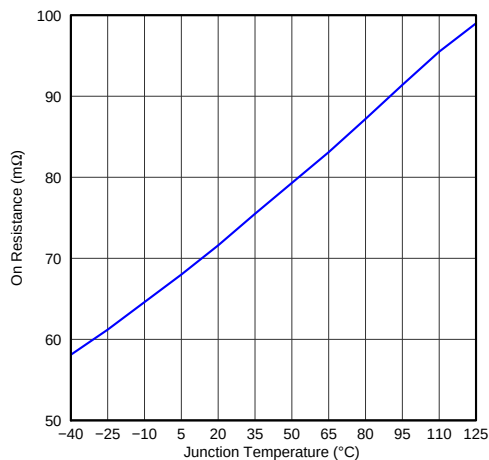
Figure 1. Power Switch On Resistance vs Temperature
