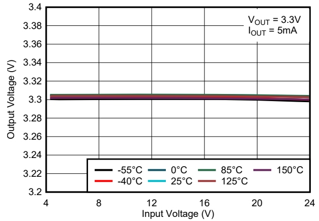
图 6-2. Line Regulation ( V_{OUT} = 3.3\text{ V} ) for New Chip
