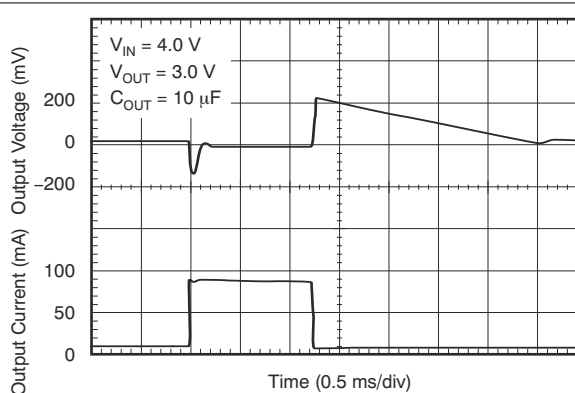
图 6-24. Load Transient Response for Legacy Chip
