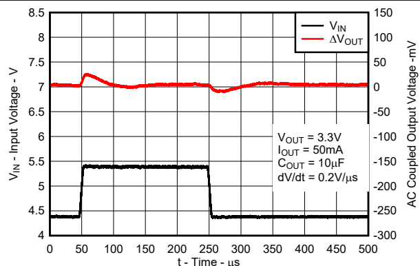
图 8-4. Line Transient Response for New Chip
