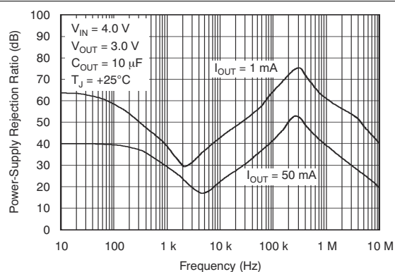
图 6-20. Power-Supply Ripple Rejection vs Frequency for Legacy Chip
