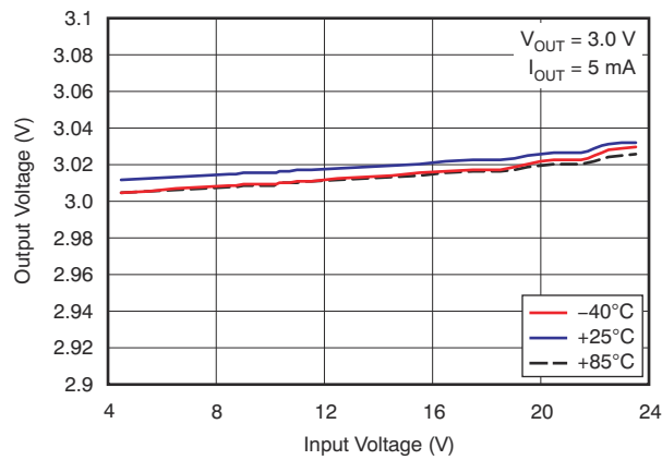
图 6-1. Line Regulation ( V_{OUT} = 3.0\text{ V} ) for Legacy Chip
