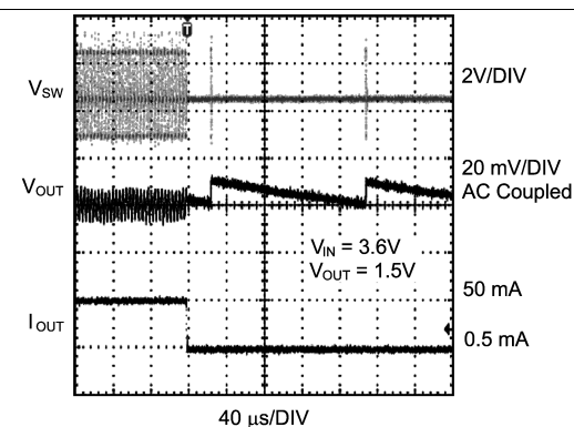
Figure 20. Load Transient Response (PWM Mode)
