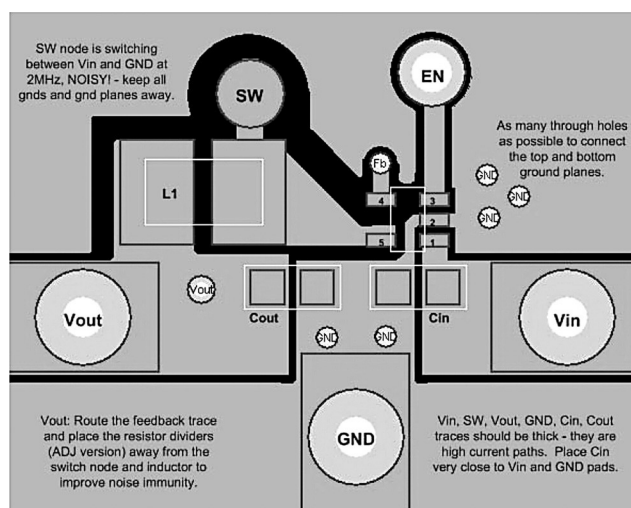
Figure 38. Top Layer Board Layout for SOT-23
