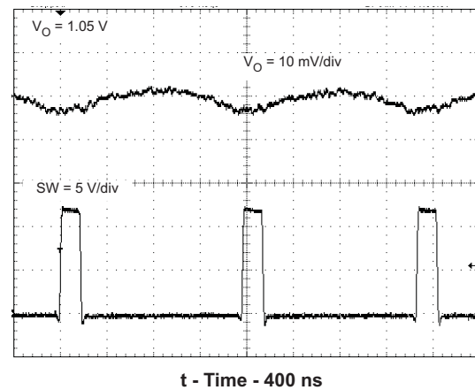
Figure 12. VOLTAGE RIPPLE AT OUTPUT ( I_O = 2\text{ A} )
