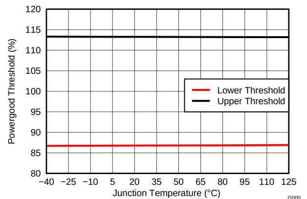
Figure 4. Power Good Threshold vs. Junction Temperature
