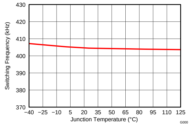
Figure 2. Switching Frequency vs. Junction Temperature
