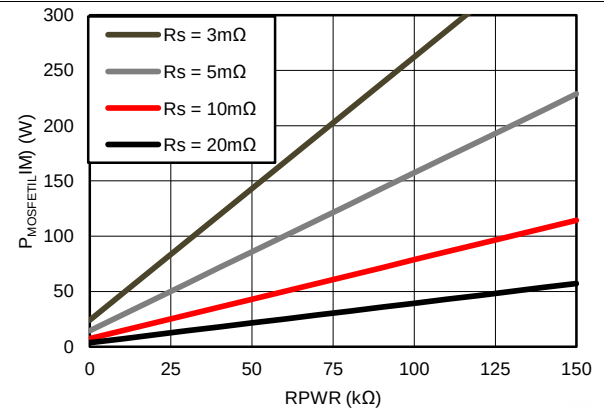
图 21. MOSFET Power Dissipation Limit vs R_{PWR} And R_S (VIN = 48 V)
