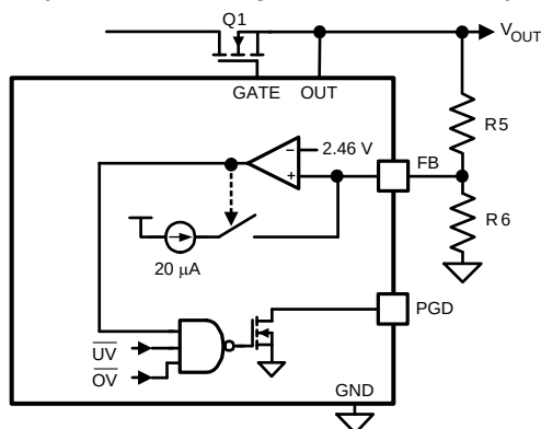
图 33. Programming the PGD Threshold
