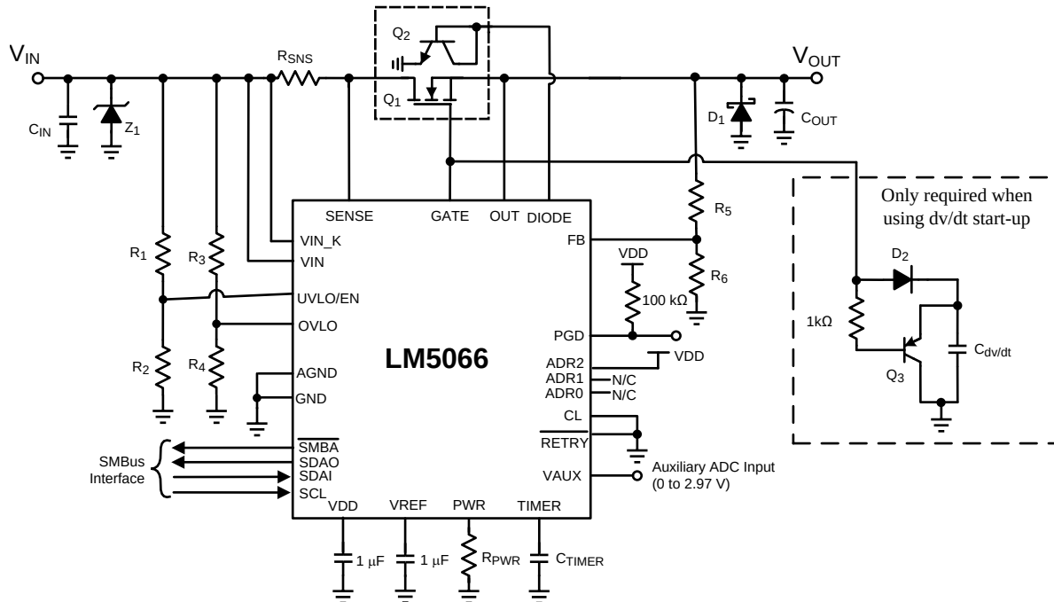
图 28. Typical Application Circuit
