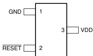
图 6-1. TLV803: DBZ Package 3-Pin SOT-23 Top View
