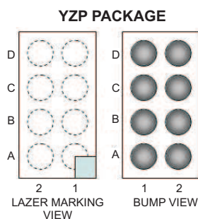
Figure 2. Bump Assignments
