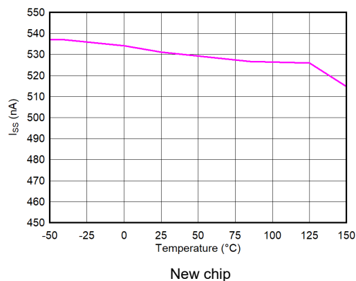
图 5-26. Soft-Start Charging Current ( I_{SS} ) vs Temperature ( T_J )
