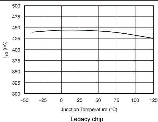
图 5-25. Soft-Start Charging Current ( I_{SS} ) vs Temperature ( T_J )
