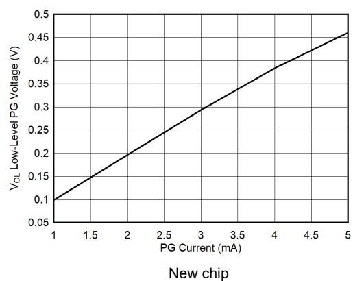
图 5-28. Low-Level PG Voltage vs Current
