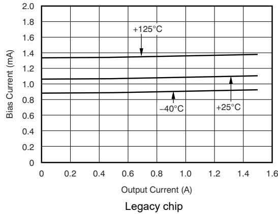
图 5-21. BIAS Pin Current vs Output Current and Temperature ( T_J )
