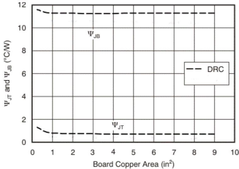
图 7-5. \Psi_{JT} and \Psi_{JB} vs Board Size
