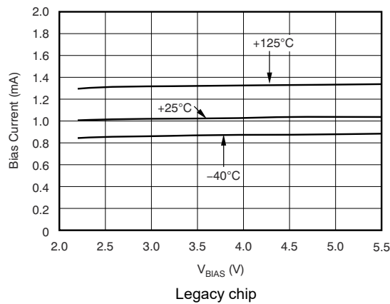
图 5-23. BIAS Pin Current vs V_{BIAS} and Temperature ( T_J )
