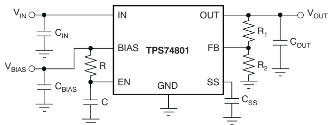
图 6-1. Soft-Start Delay Using an RC Circuit to Enable the Device
