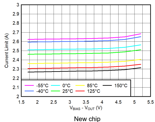
图 5-30. Current Limit vs ( V_{BIAS} - V_{OUT} )
