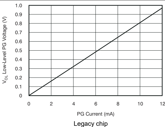
图 5-27. Low-Level PG Voltage vs Current
