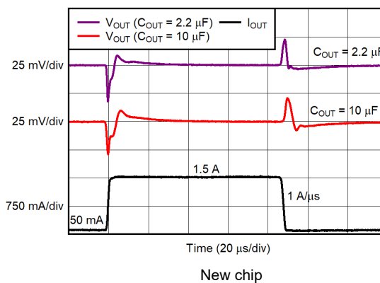
图 5-36. Output Load Transient Response
