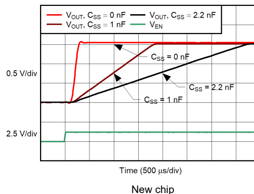
图 5-38. Turn-On Response
