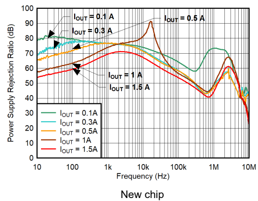
图 5-16. V_{IN} PSRR vs Frequency
