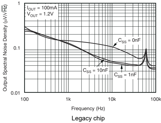
图 5-19. Noise Spectral Density
