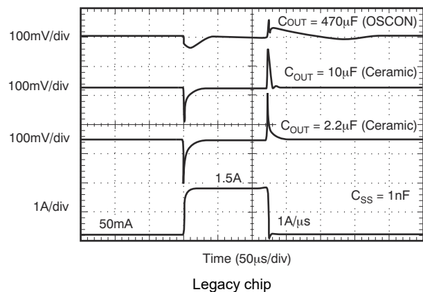
图 5-35. Output Load Transient Response
