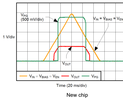
图 5-40. Power-Up, Power-Down
