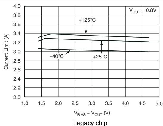
图 5-29. Current Limit vs ( V_{BIAS} - V_{OUT} )
