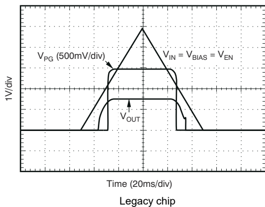
图 5-39. Power-Up, Power-Down
