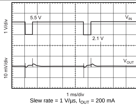
Figure 21. Line Transient Response
