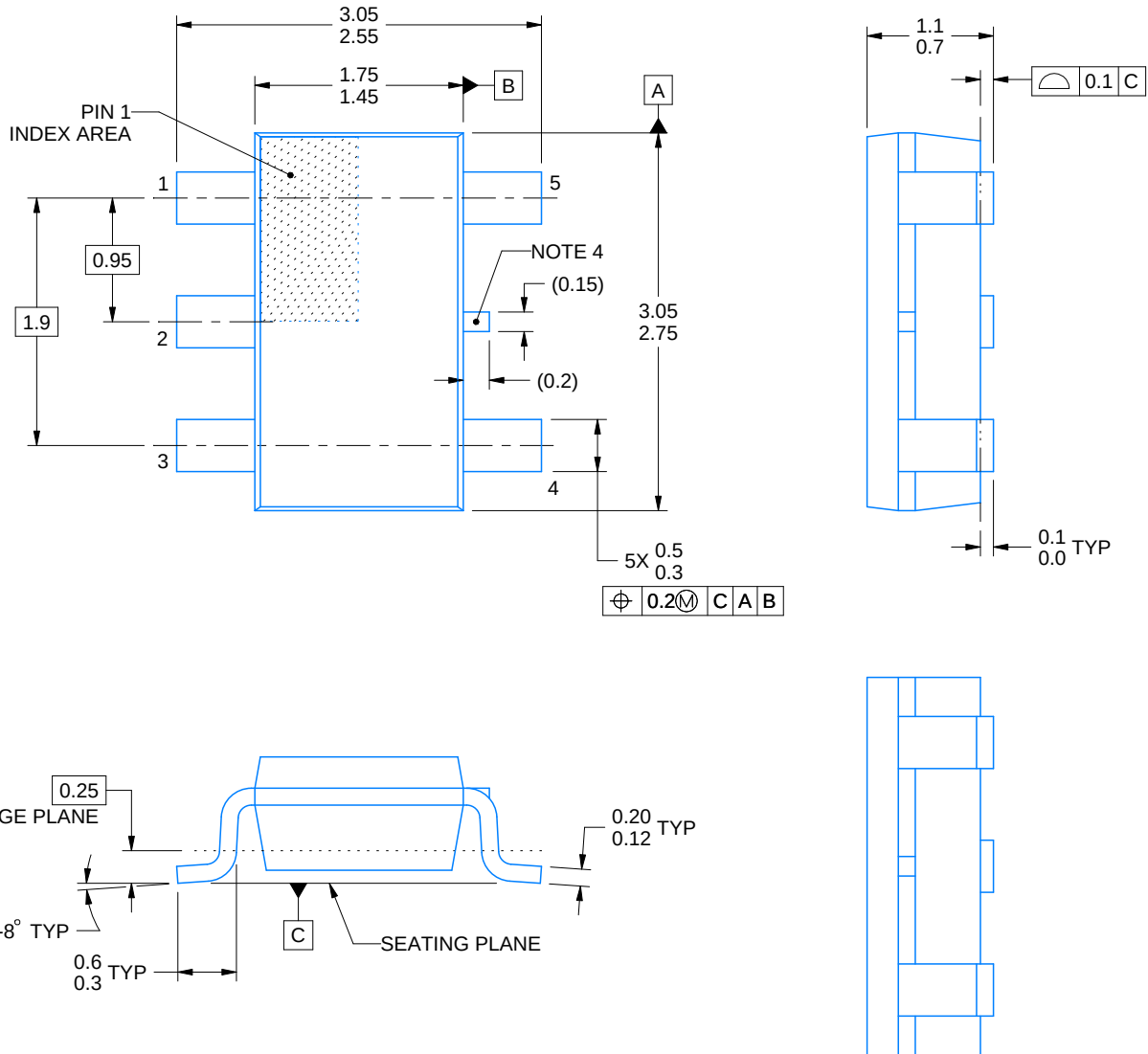
ALTERNATIVE PACKAGE SINGULATION VIEW
