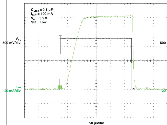
图 5-22. t_{ON} Response
