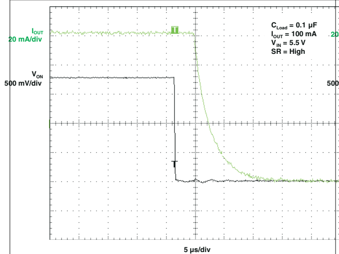
图 5-18. t_{OFF} Response
