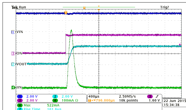
图 8-2. Inrush Current with SR = Low
