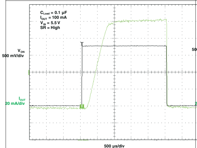
图 5-14. t_{ON} Response
