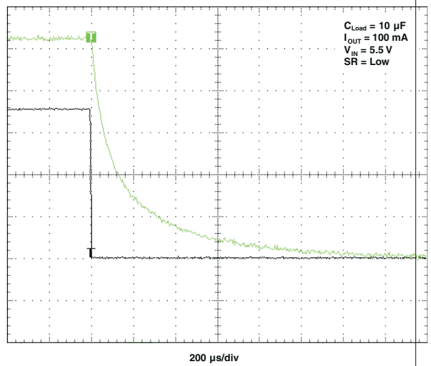
图 5-27. t_{OFF} Response
