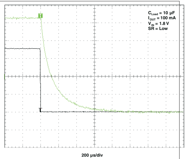
图 5-25. t_{OFF} Response
