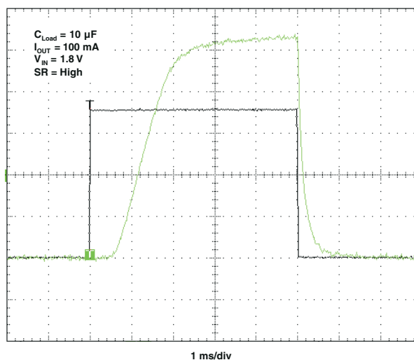
图 5-13. t_{ON} Response
