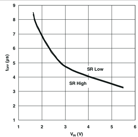
图 5-11. Off Time vs Input Voltage
