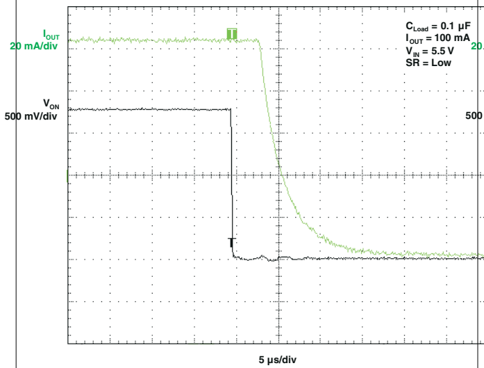
图 5-26. t_{OFF} Response
