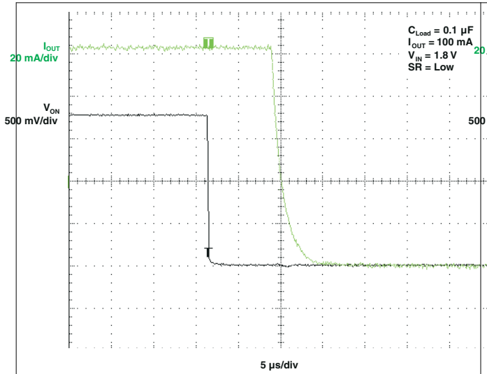
图 5-24. t_{OFF} Response
