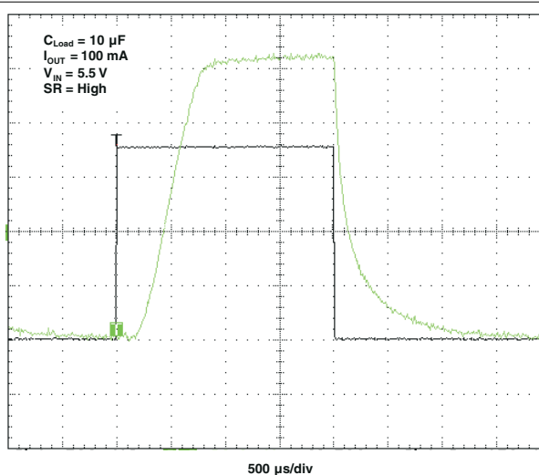
图 5-15. t_{ON} Response
