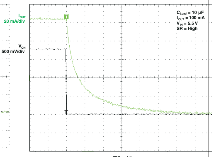
图 5-19. t_{OFF} Response
