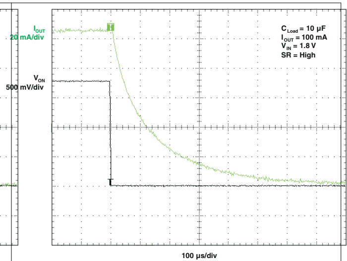
图 5-17. t_{OFF} Response
