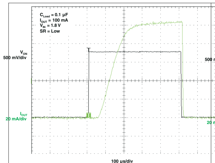
图 5-20. t_{ON} Response
