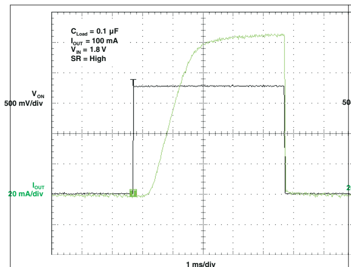
图 5-12. t_{ON} Response
