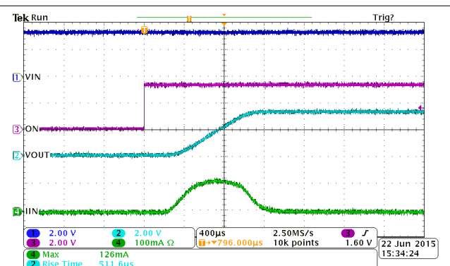
图 8-3. Inrush Current with SR = High
