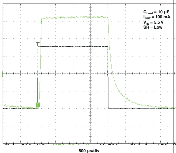
图 5-23. t_{ON} Response
