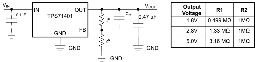
图 7-2. TPS714 Adjustable LDO Regulator Programming
