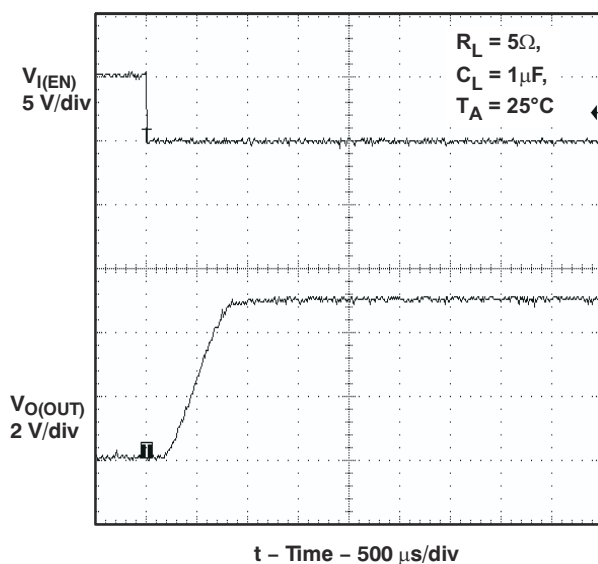
图 6-2. Turnon Delay and Rise Time With 1-μF Load
