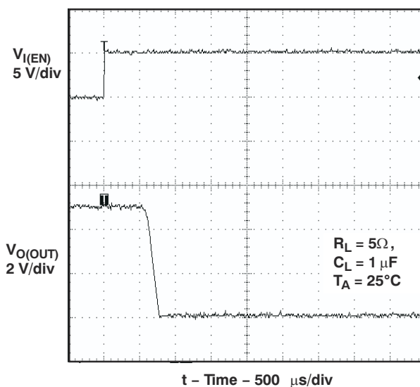
图 6-3. Turnoff Delay and Fall Time With 1-μF Load
