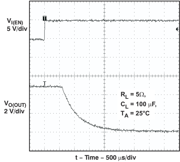
图 6-5. Turnoff Delay and Fall Time With 100-μF Load
