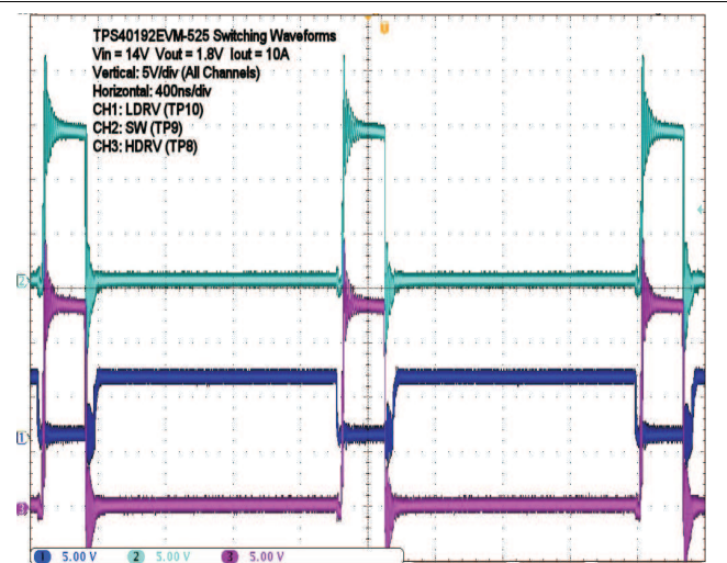
Figure 22. Switching Waveforms
