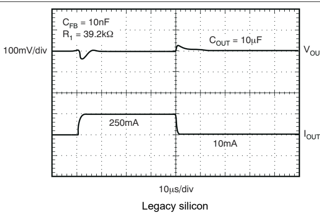
图 5-41. TPS73701 Load Transient, Adjustable Version
