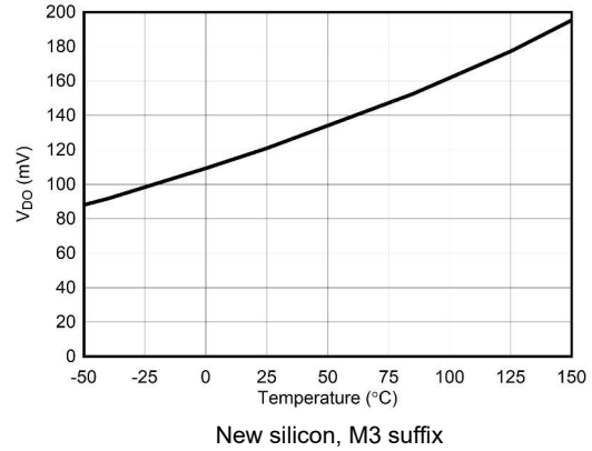
图 5-8. Dropout Voltage vs Temperature
