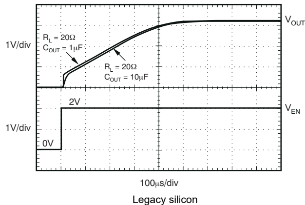
图 5-32. TPS73701 Turn-On Response
