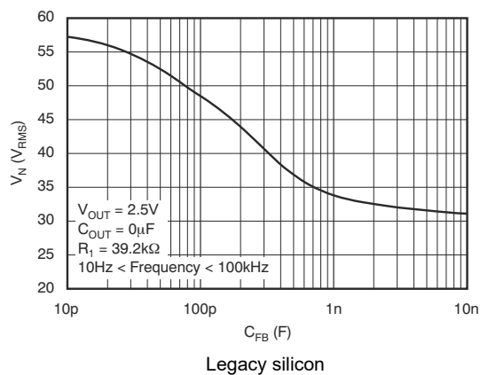
图 5-39. TPS73701 RMS Noise Voltage vs C_{FB}
