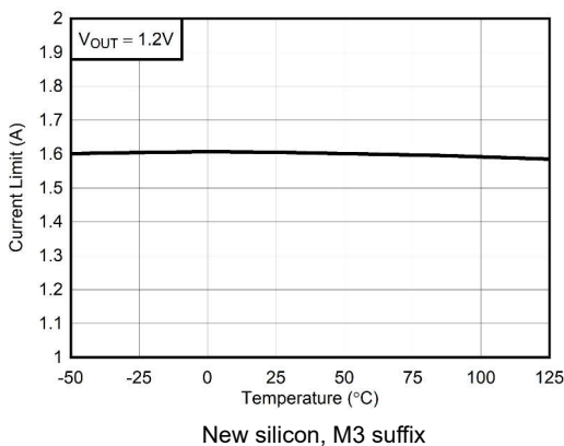
图 5-21. Current Limit vs Temperature
