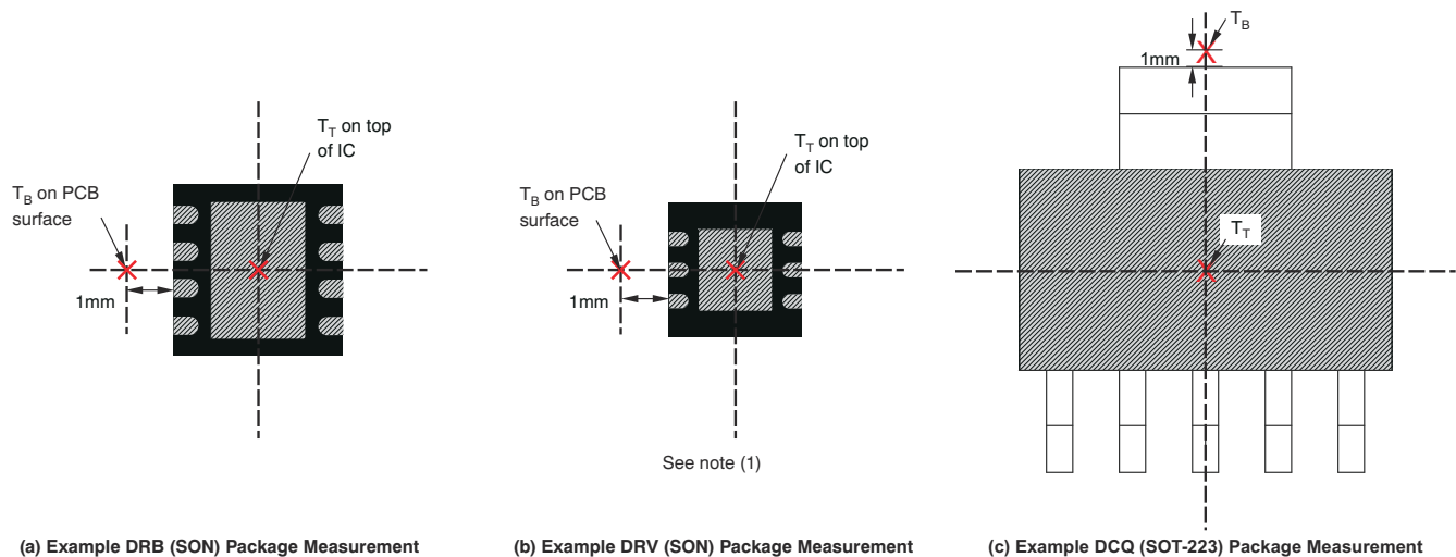
图 7-8. Measuring Points for T_T and T_B
