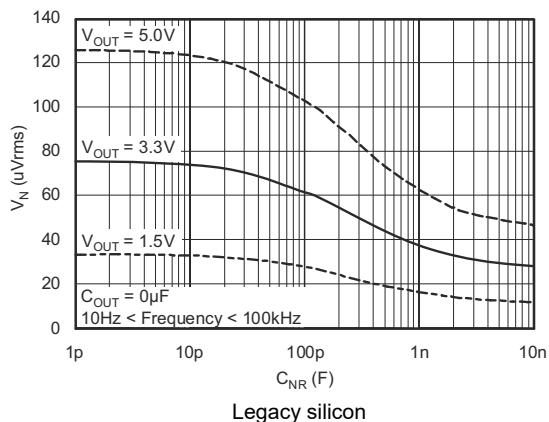
图 5-29. RMS Noise Voltage vs C_{NR}
