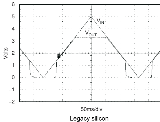
图 7-5. TPS73701, V_{OUT} = 3.3\text{-V} Power-Up and Power-Down
