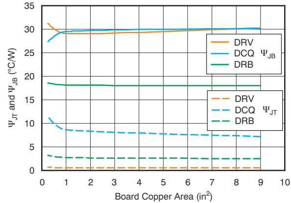
图 7-7. \Psi_{JT} and \Psi_{JB} vs Board Size
