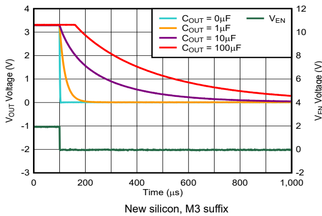
图 5-35. TPS73701 Turn-Off Response
