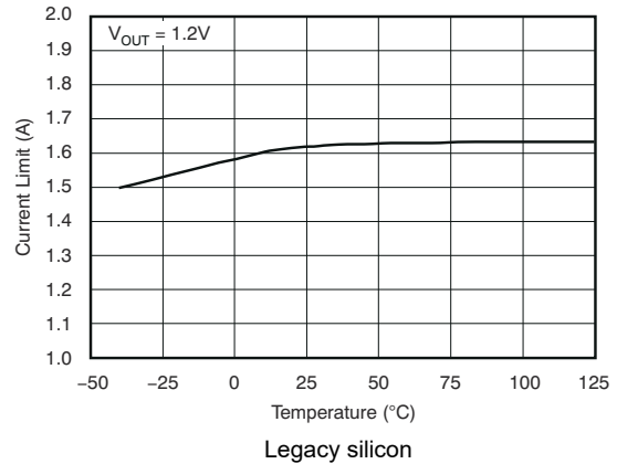
图 5-20. Current Limit vs Temperature
