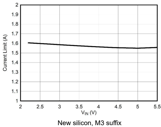
图 5-19. Current Limit vs V_{IN}
