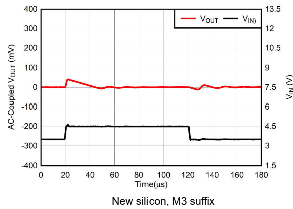
图 5-43. TPS73701 Line Transient, Adjustable Version
