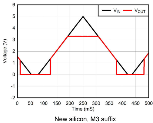
图 5-37. TPS73701, V_{OUT} = 3.3\text{-V} Power-Up and Power-Down
