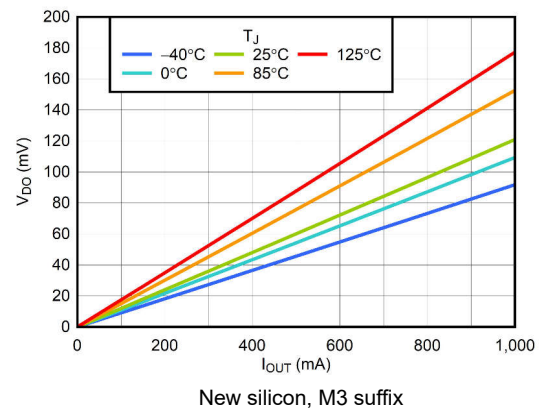
图 5-6. Dropout Voltage vs Output Current
