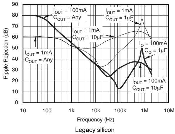
图 7-3. PSRR (Ripple Rejection) vs Frequency
