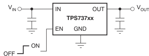
图 7-1. Typical Application Circuit for Fixed-Voltage Versions
