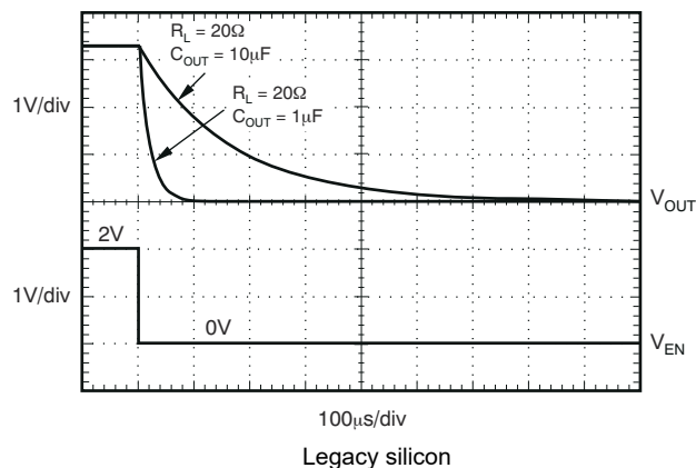
图 5-34. TPS73701 Turn-Off Response
