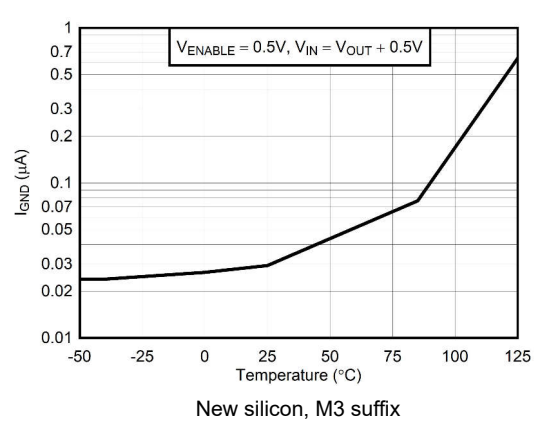
图 5-16. Ground Pin Current in Shutdown vs Temperature
