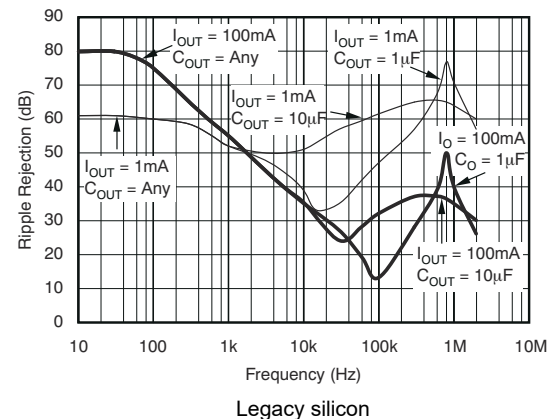
图 5-22. PSRR (Ripple Rejection) vs Frequency
