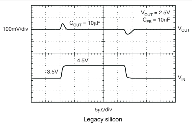
图 5-42. TPS73701 Line Transient, Adjustable Version
