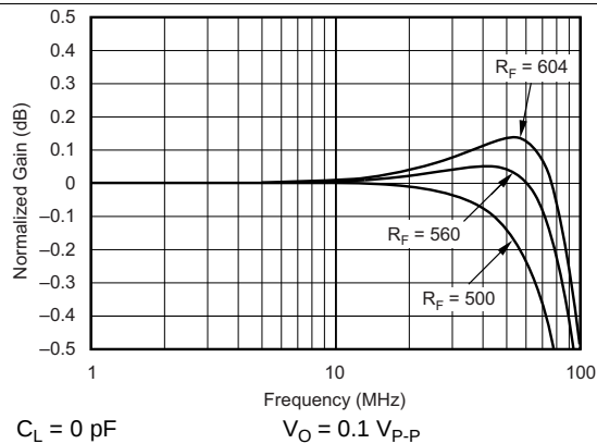
图 6. 0.1-dB Gain Flatness for Various R_F Values?
