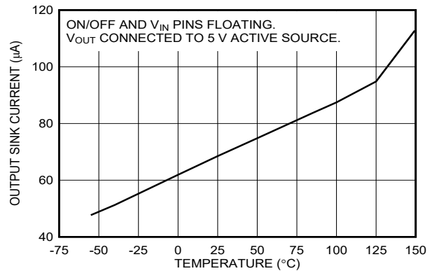
图 5-24. Output Reverse Leakage vs Temperature (New Chip)
