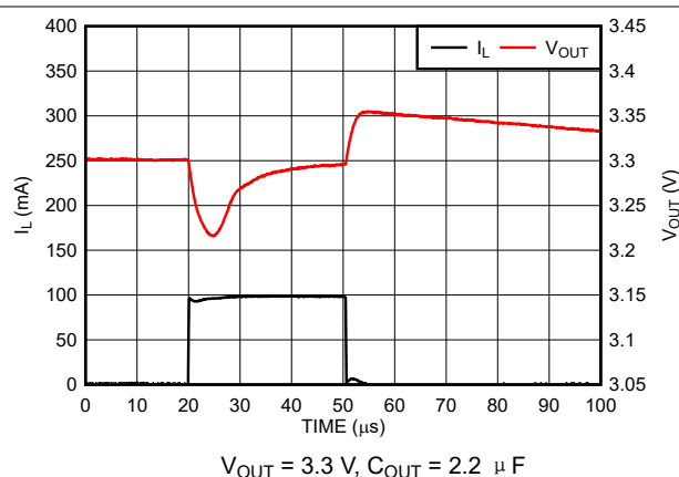
图 5-15. Load Transient Response (New Chip)
