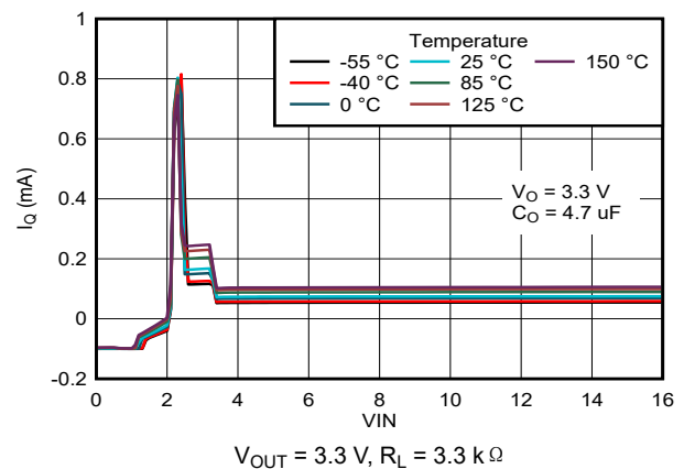
图 5-12. Input Current vs Input Voltage ( V_{IN} ) (New Chip)
