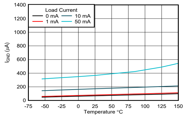
图 5-10. Ground Pin Current ( I_{GND} ) vs Temperature (New Chip)
