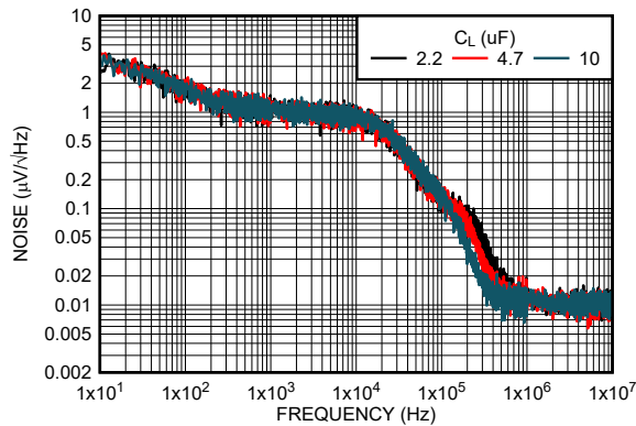
图 5-23. Output Noise Density vs Output Capacitor ( C_L ) Frequency (New Chip)
