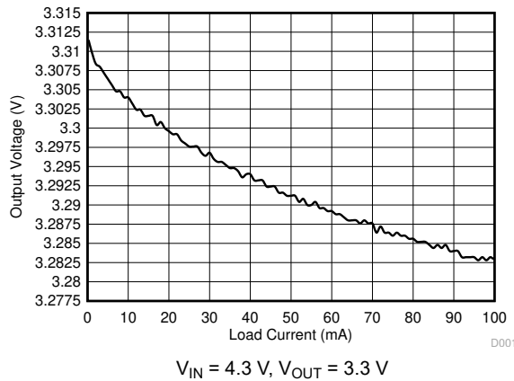
图 5-1. Output Voltage vs Load Current (Legacy Chip)
