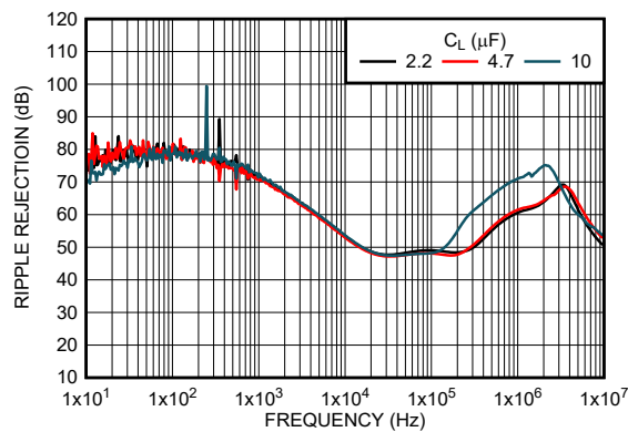
图 5-21. Ripple Rejection vs Output Capacitor ( C_L ) and Frequency (New Chip)
