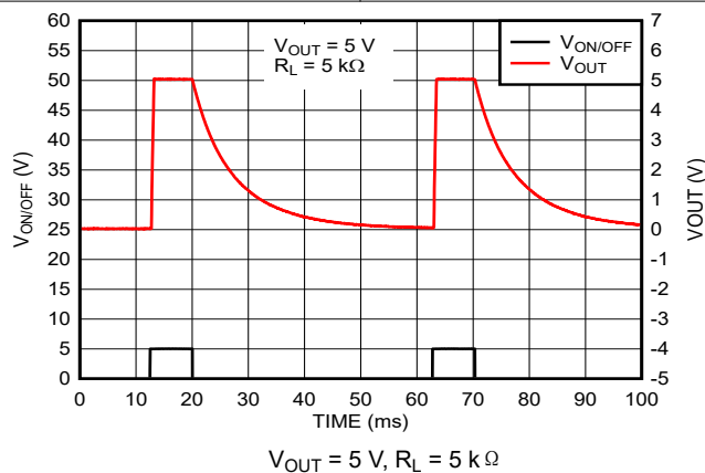
图 7-11. Turn-off Waveform (New Chip)
