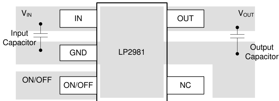
图 9-1. Recommended Layout
