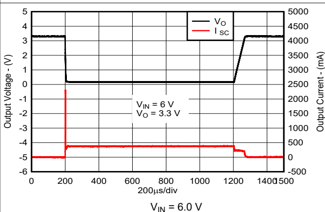
图 5-16. Short Circuit Current vs Time (New Chip)
