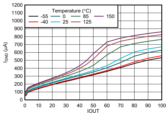
图 5-11. Ground Pin Current ( I_{GND} ) vs Load Current (New Chip)
