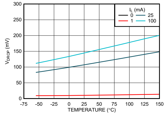
图 5-8. Dropout Voltage ( V_{DO} ) vs Temperature (New Chip)
