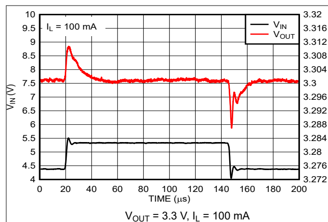
图 7-7. Line Transient Response (New Chip)
