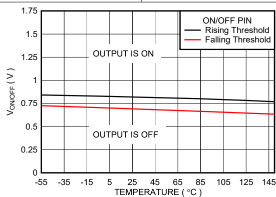
图 5-29. ON/ OFF Threshold vs Temperature (New Chip)
