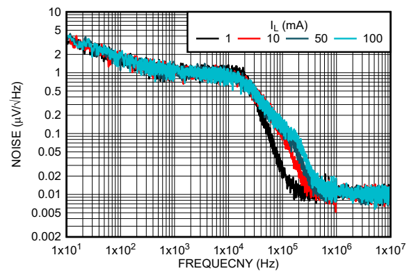
图 5-22. Output Noise Density vs Load Current ( I_L ) Frequency (New Chip)
