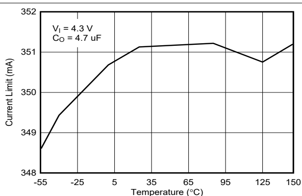
图 5-18. Instantaneous Short Circuit Current vs Temperature (New Chip)
