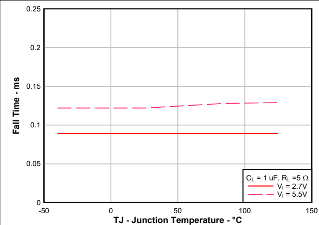
图 6-4. Fall Time vs Junction Temperature
