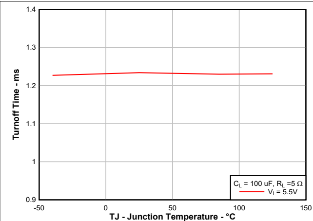
图 6-2. Turnoff Time vs Junction Temperature
