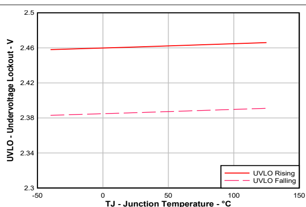
图 6-36. Undervoltage Lockout vs Junction Temperature
