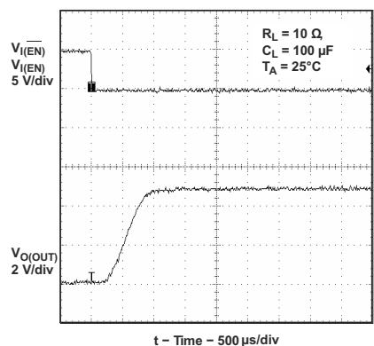
图 6-19. Turnon Delay and Rise Time With 100-μF Load
