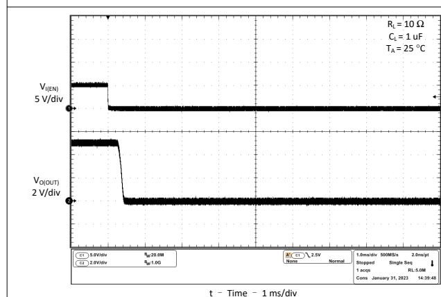
图 6-39. Turnoff Delay and Fall Time With 1-μF Load
